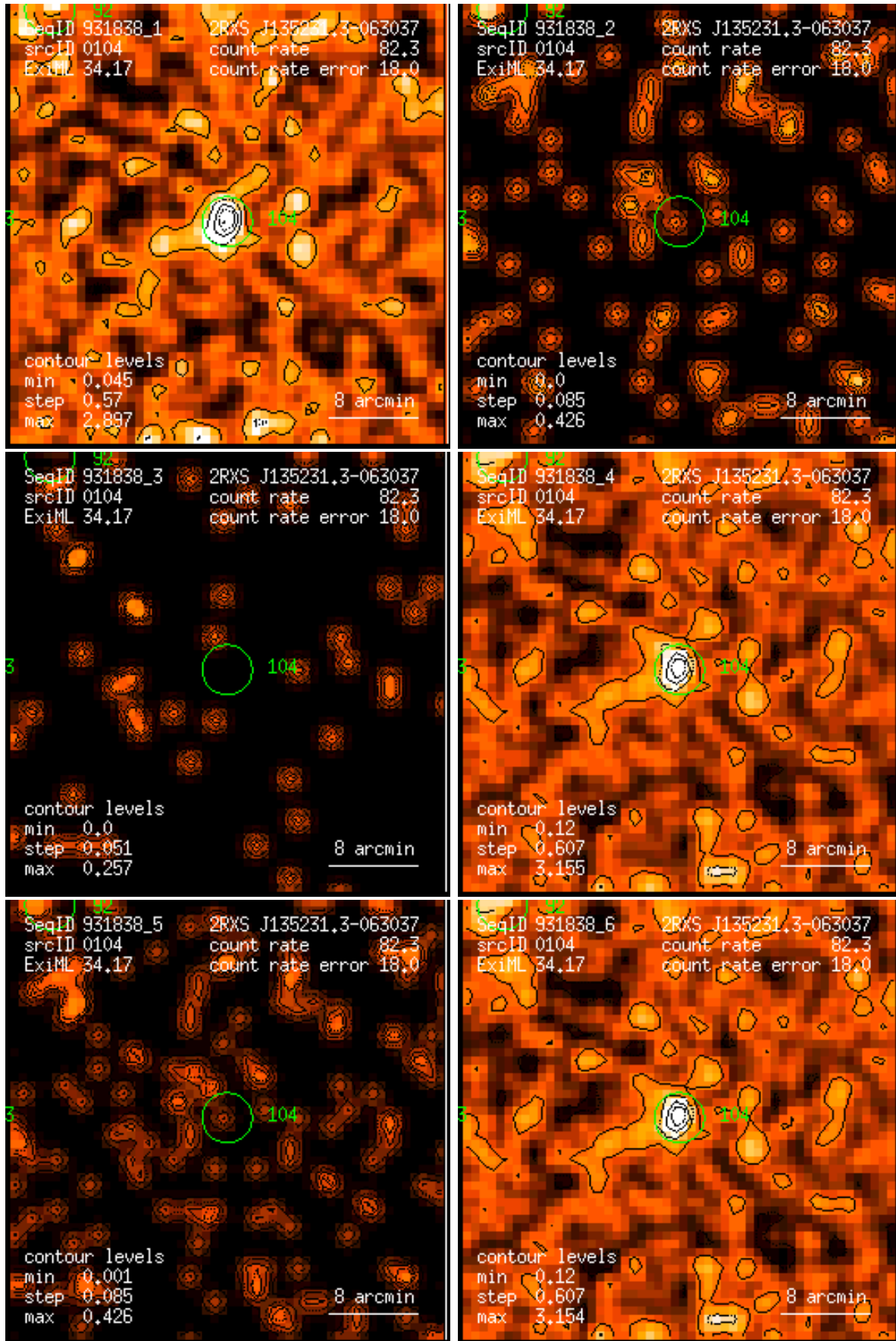
Figure 104: RASS 931838: detection 0104: band rate images, Gaussian filter: (1) PSPC channels 11 – 41, (2) 52 – 90, (3) 91 – 201, (4) 11 – 235, (5) 52 – 201, (6) 11 – 201. Broad band rates in counts/ks. Band rate contour levels in counts/ks/arcmin 2 .
