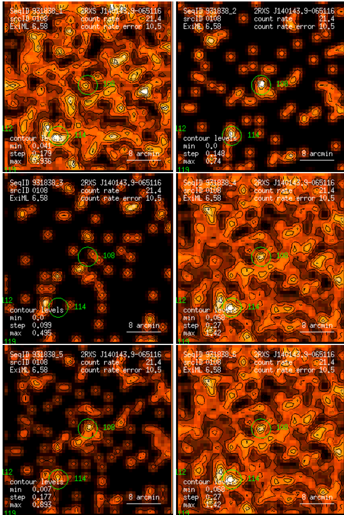
Figure 108: RASS 931838: detection 0108: band rate images, Gaussian filter: (1) PSPC channels 11 – 41, (2) 52 – 90, (3) 91 – 201, (4) 11 – 235, (5) 52 – 201, (6) 11 – 201. Broad band rates in counts/ks. Band rate contour levels in counts/ks/arcmin 2 .
