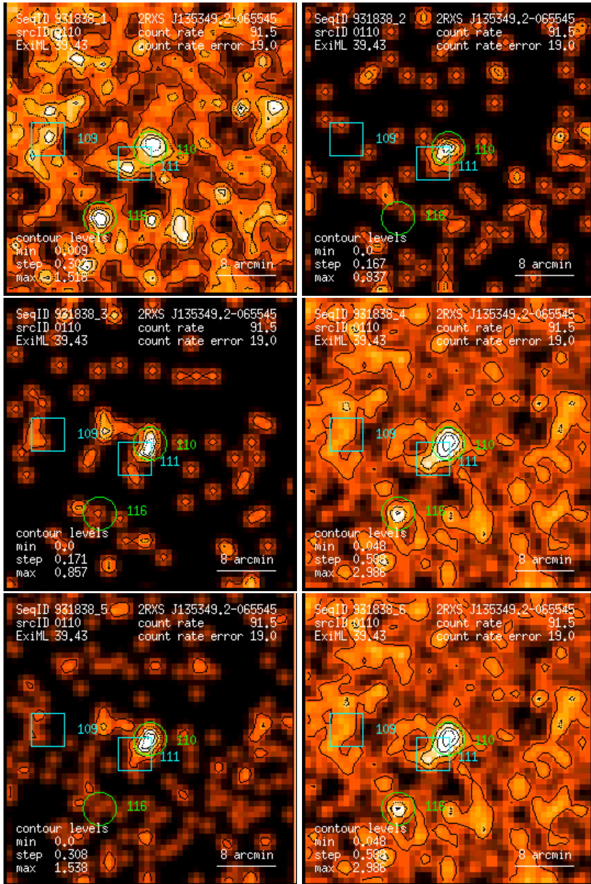
Figure 110: RASS 931838: detection 0110: band rate images, Gaussian filter: (1) PSPC channels 11 – 41, (2) 52 – 90, (3) 91 – 201, (4) 11 – 235, (5) 52 – 201, (6) 11 – 201. Broad band rates in counts/ks. Band rate contour levels in counts/ks/arcmin 2 .
