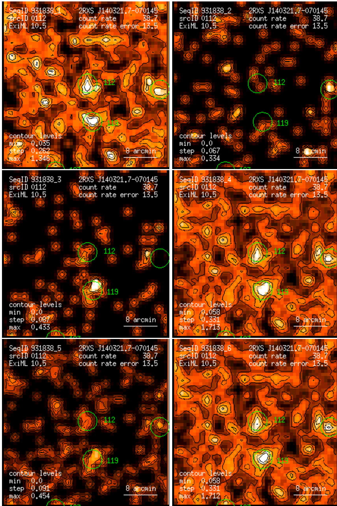
Figure 112: RASS 931838: detection 0112: band rate images, Gaussian filter: (1) PSPC channels 11 – 41, (2) 52 – 90, (3) 91 – 201, (4) 11 – 235, (5) 52 – 201, (6) 11 – 201. Broad band rates in counts/ks. Band rate contour levels in counts/ks/arcmin 2 .
