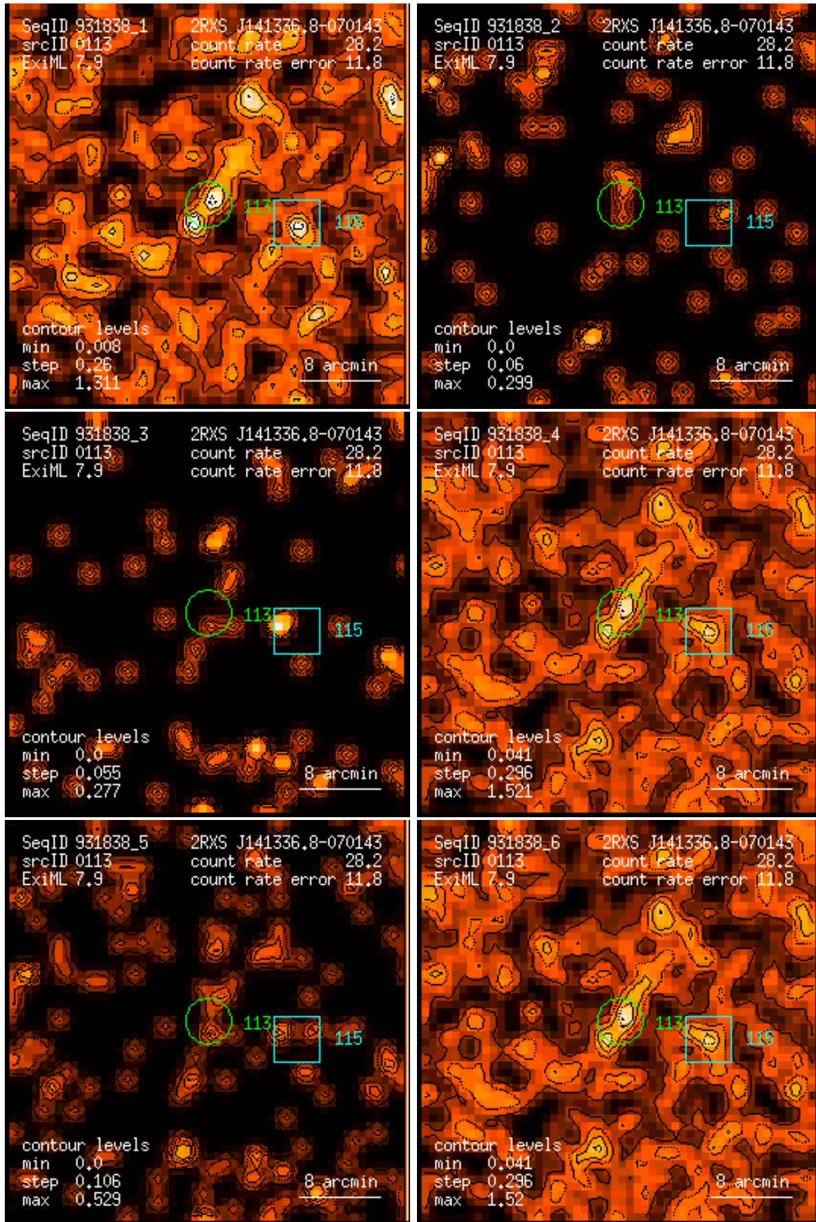
Figure 113: RASS 931838: detection 0113: band rate images, Gaussian filter: (1) PSPC channels 11 – 41, (2) 52 – 90, (3) 91 – 201, (4) 11 – 235, (5) 52 – 201, (6) 11 – 201. Broad band rates in counts/ks. Band rate contour levels in counts/ks/arcmin 2 .
