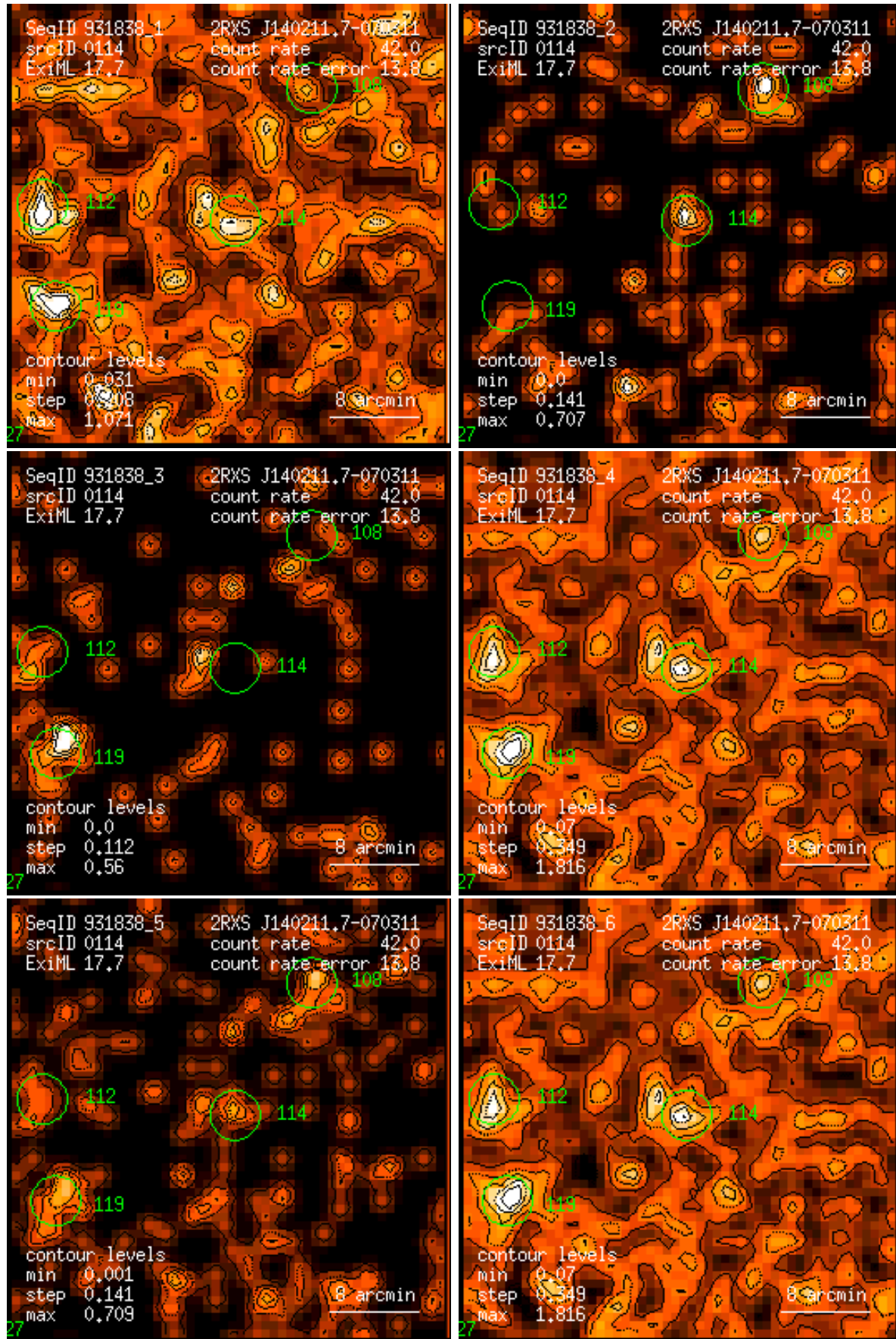
Figure 114: RASS 931838: detection 0114: band rate images, Gaussian filter: (1) PSPC channels 11 – 41, (2) 52 – 90, (3) 91 – 201, (4) 11 – 235, (5) 52 – 201, (6) 11 – 201. Broad band rates in counts/ks. Band rate contour levels in counts/ks/arcmin 2 .
