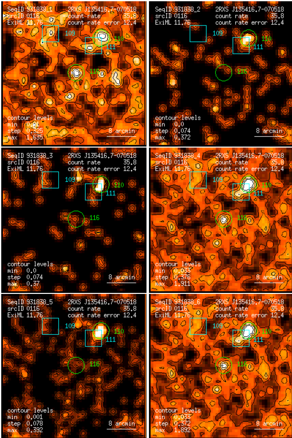
Figure 116: RASS 931838: detection 0116: band rate images, Gaussian filter: (1) PSPC channels 11 – 41, (2) 52 – 90, (3) 91 – 201, (4) 11 – 235, (5) 52 – 201, (6) 11 – 201. Broad band rates in counts/ks. Band rate contour levels in counts/ks/arcmin 2 .
