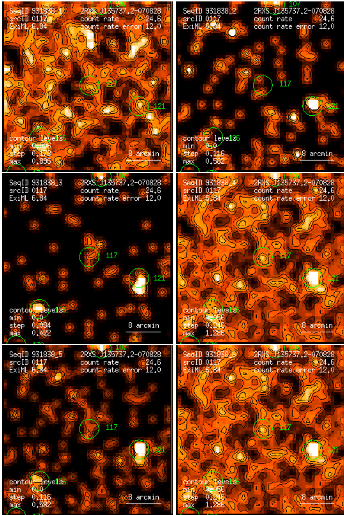
Figure 117: RASS 931838: detection 0117: band rate images, Gaussian filter: (1) PSPC channels 11 – 41, (2) 52 – 90, (3) 91 – 201, (4) 11 – 235, (5) 52 – 201, (6) 11 – 201. Broad band rates in counts/ks. Band rate contour levels in counts/ks/arcmin 2 .
