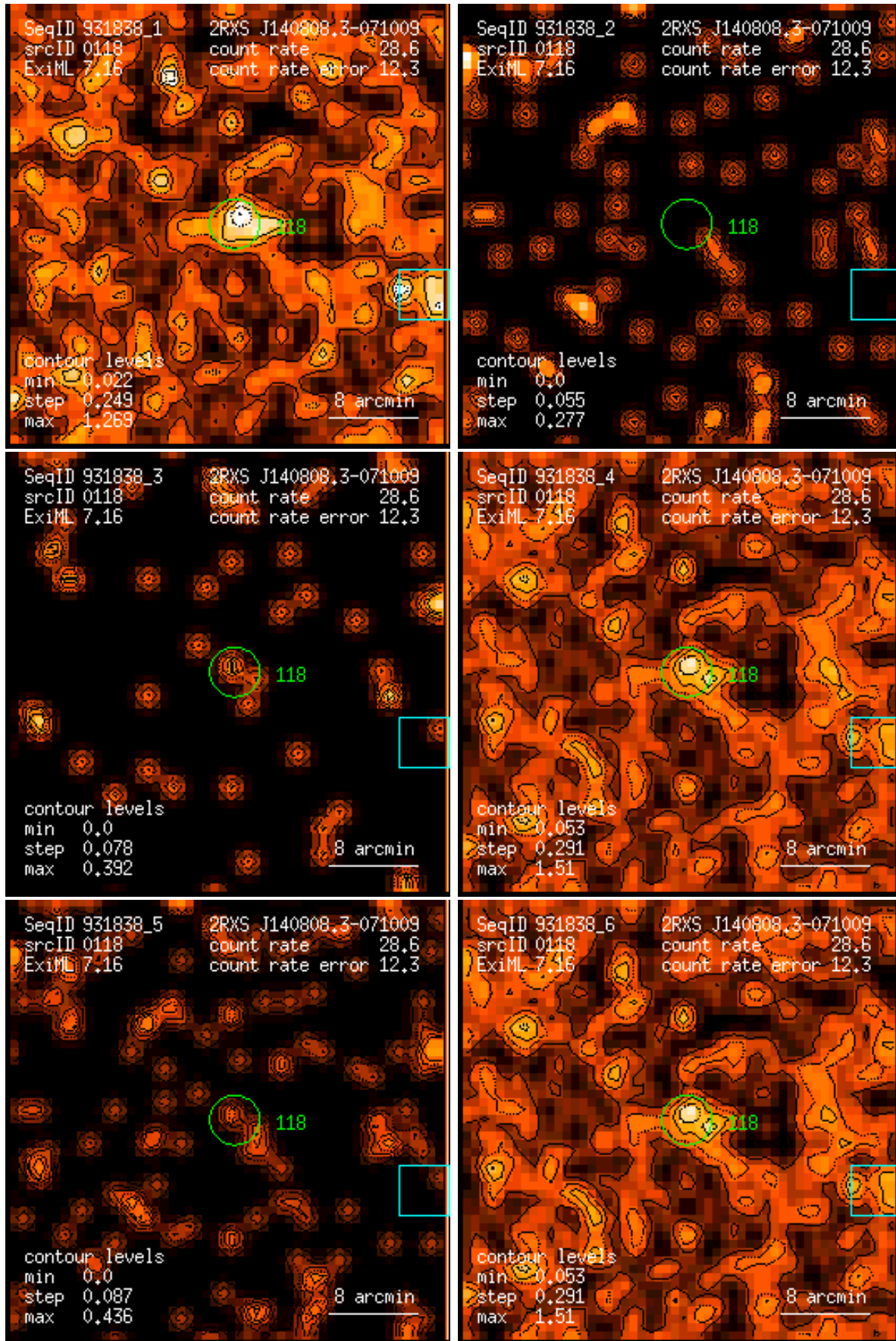
Figure 118: RASS 931838: detection 0118: band rate images, Gaussian filter: (1) PSPC channels 11 – 41, (2) 52 – 90, (3) 91 – 201, (4) 11 – 235, (5) 52 – 201, (6) 11 – 201. Broad band rates in counts/ks. Band rate contour levels in counts/ks/arcmin 2 .
