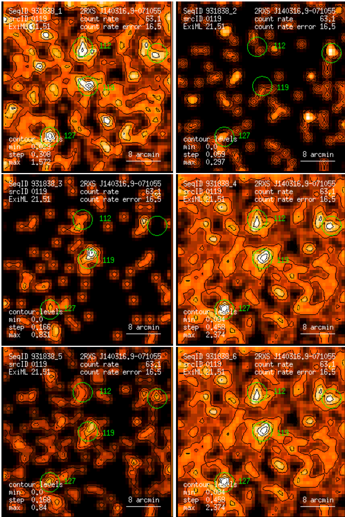
Figure 119: RASS 931838: detection 0119: band rate images, Gaussian filter: (1) PSPC channels 11 – 41, (2) 52 – 90, (3) 91 – 201, (4) 11 – 235, (5) 52 – 201, (6) 11 – 201. Broad band rates in counts/ks. Band rate contour levels in counts/ks/arcmin 2 .
