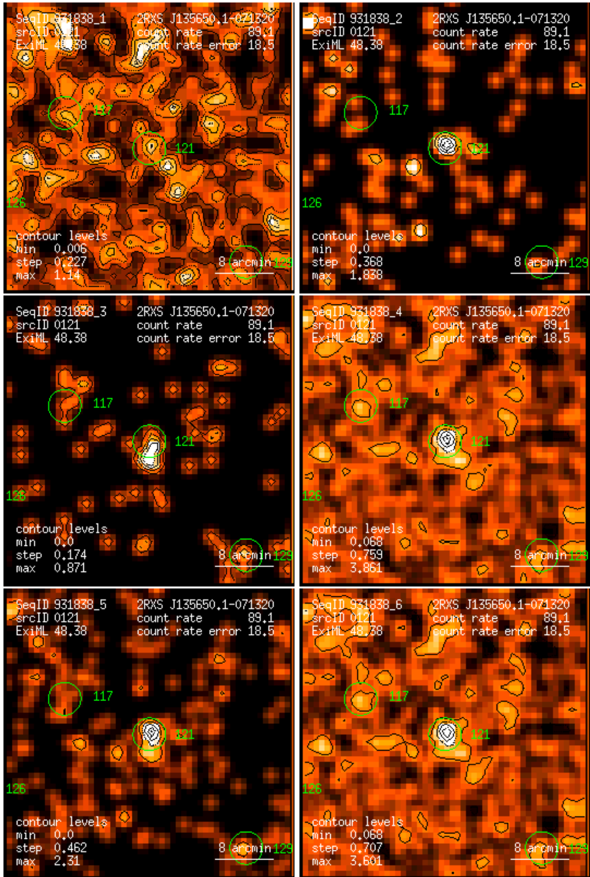
Figure 121: RASS 931838: detection 0121: band rate images, Gaussian filter: (1) PSPC channels 11 – 41, (2) 52 – 90, (3) 91 – 201, (4) 11 – 235, (5) 52 – 201, (6) 11 – 201. Broad band rates in counts/ks. Band rate contour levels in counts/ks/arcmin 2 .
