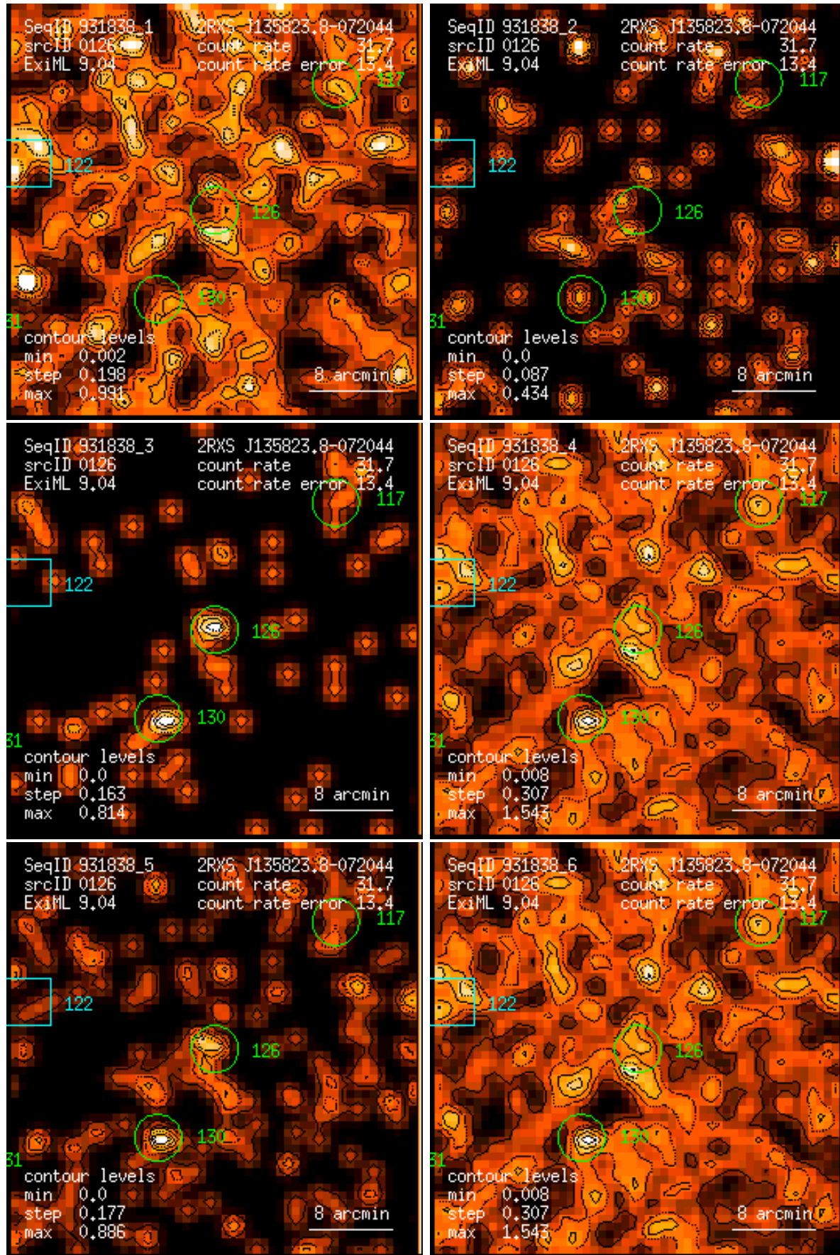
Figure 126: RASS 931838: detection 0126: band rate images, Gaussian filter: (1) PSPC channels 11 – 41, (2) 52 – 90, (3) 91 – 201, (4) 11 – 235, (5) 52 – 201, (6) 11 – 201. Broad band rates in counts/ks. Band rate contour levels in counts/ks/arcmin 2 .
