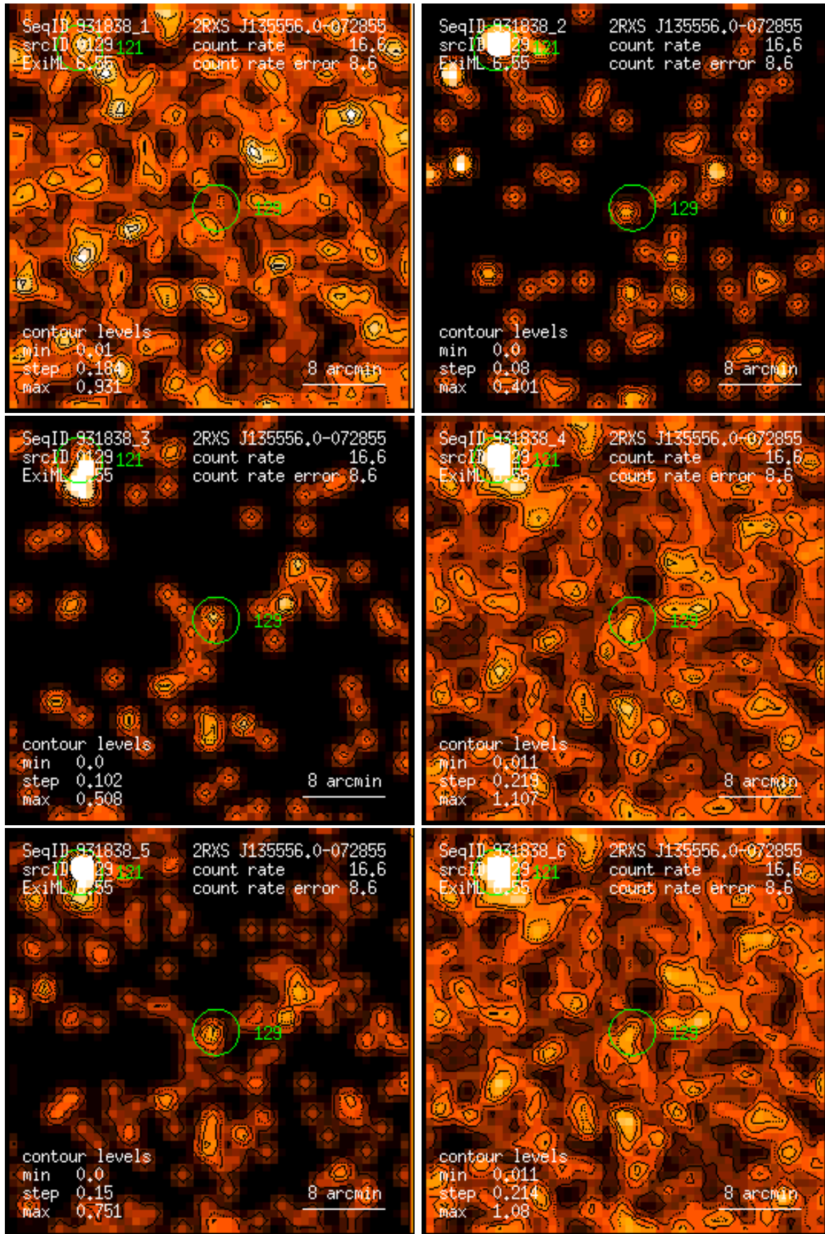
Figure 129: RASS 931838: detection 0129: band rate images, Gaussian filter: (1) PSPC channels 11 – 41, (2) 52 – 90, (3) 91 – 201, (4) 11 – 235, (5) 52 – 201, (6) 11 – 201. Broad band rates in counts/ks. Band rate contour levels in counts/ks/arcmin 2 .
