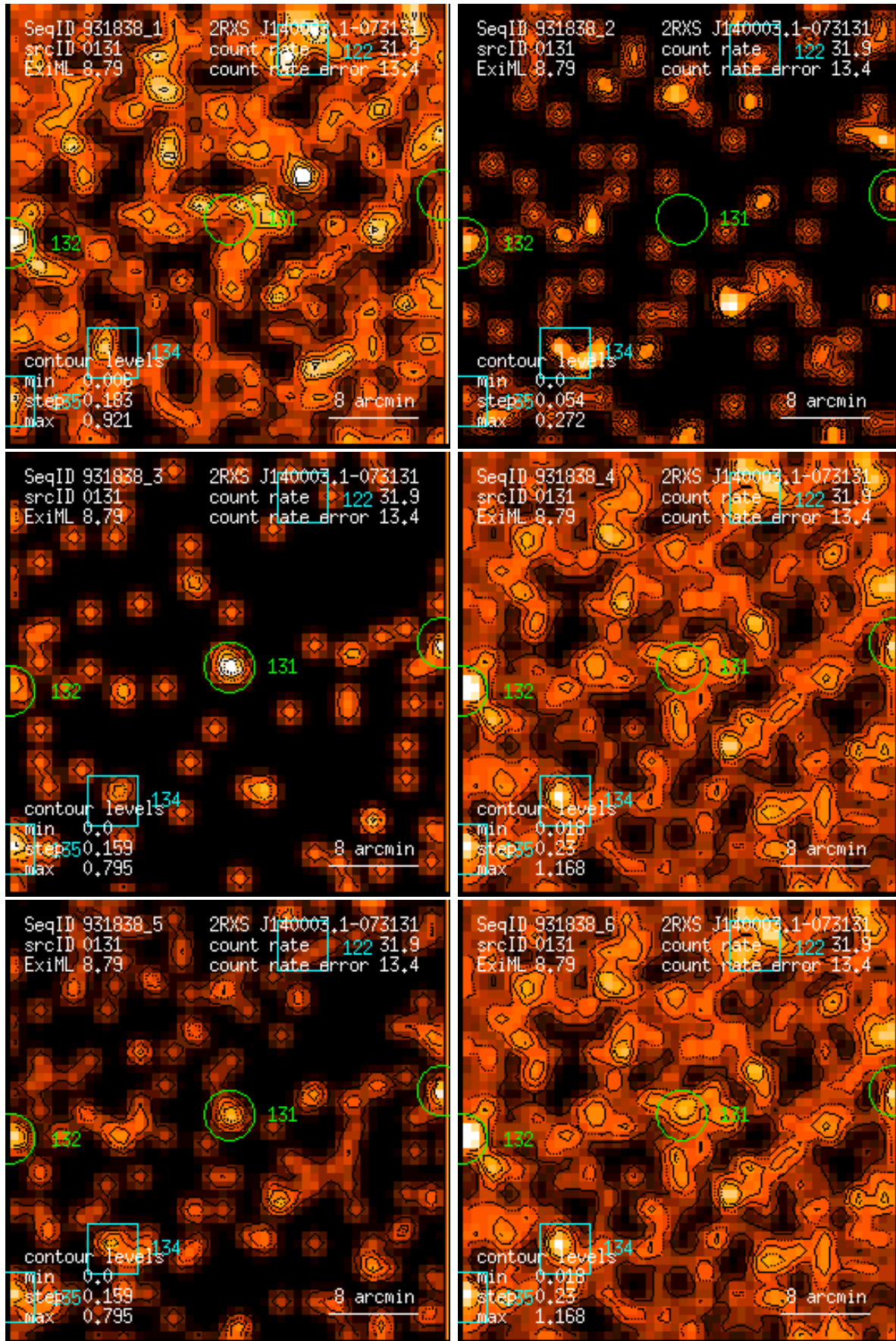
Figure 131: RASS 931838: detection 0131: band rate images, Gaussian filter: (1) PSPC channels 11 – 41, (2) 52 – 90, (3) 91 – 201, (4) 11 – 235, (5) 52 – 201, (6) 11 – 201. Broad band rates in counts/ks. Band rate contour levels in counts/ks/arcmin 2 .
