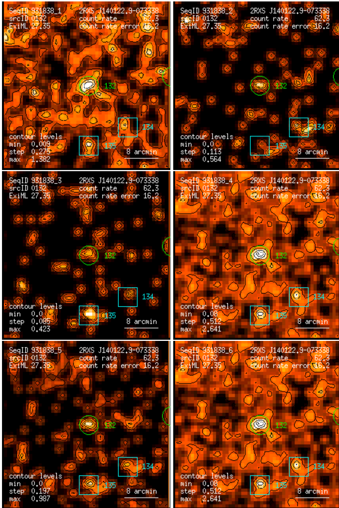
Figure 132: RASS 931838: detection 0132: band rate images, Gaussian filter: (1) PSPC channels 11 – 41, (2) 52 – 90, (3) 91 – 201, (4) 11 – 235, (5) 52 – 201, (6) 11 – 201. Broad band rates in counts/ks. Band rate contour levels in counts/ks/arcmin 2 .
