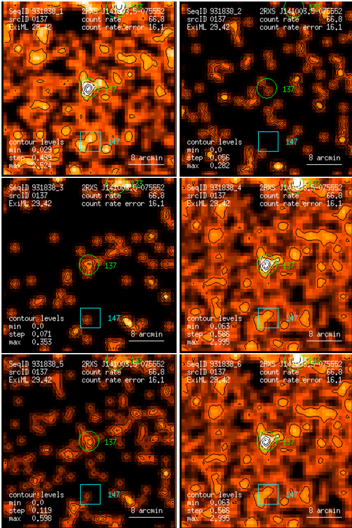
Figure 137: RASS 931838: detection 0137: band rate images, Gaussian filter: (1) PSPC channels 11 – 41, (2) 52 – 90, (3) 91 – 201, (4) 11 – 235, (5) 52 – 201, (6) 11 – 201. Broad band rates in counts/ks. Band rate contour levels in counts/ks/arcmin 2 .
