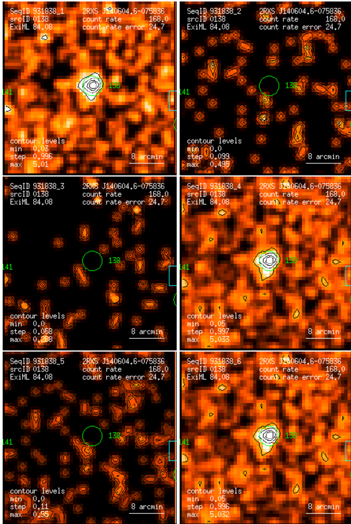
Figure 138: RASS 931838: detection 0138: band rate images, Gaussian filter: (1) PSPC channels 11 – 41, (2) 52 – 90, (3) 91 – 201, (4) 11 – 235, (5) 52 – 201, (6) 11 – 201. Broad band rates in counts/ks. Band rate contour levels in counts/ks/arcmin 2 .
