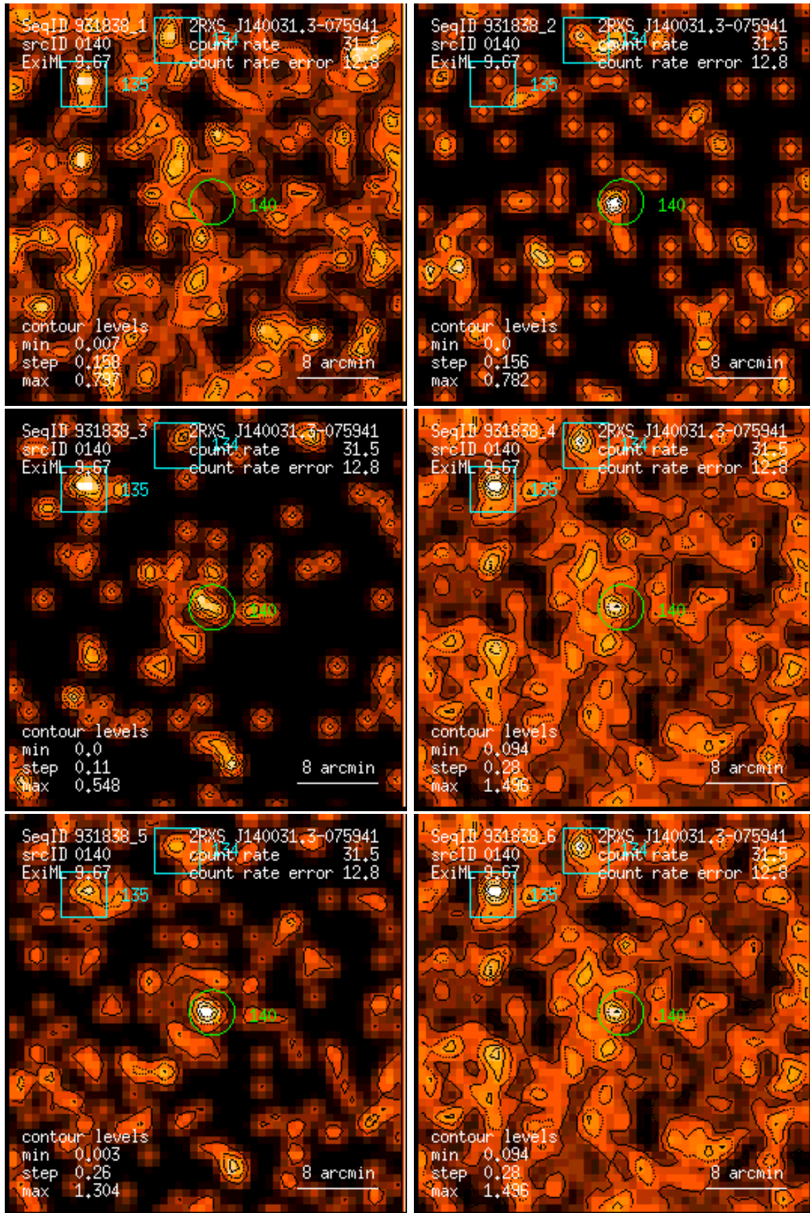
Figure 140: RASS 931838: detection 0140: band rate images, Gaussian filter: (1) PSPC channels 11 – 41, (2) 52 – 90, (3) 91 – 201, (4) 11 – 235, (5) 52 – 201, (6) 11 – 201. Broad band rates in counts/ks. Band rate contour levels in counts/ks/arcmin 2 .
