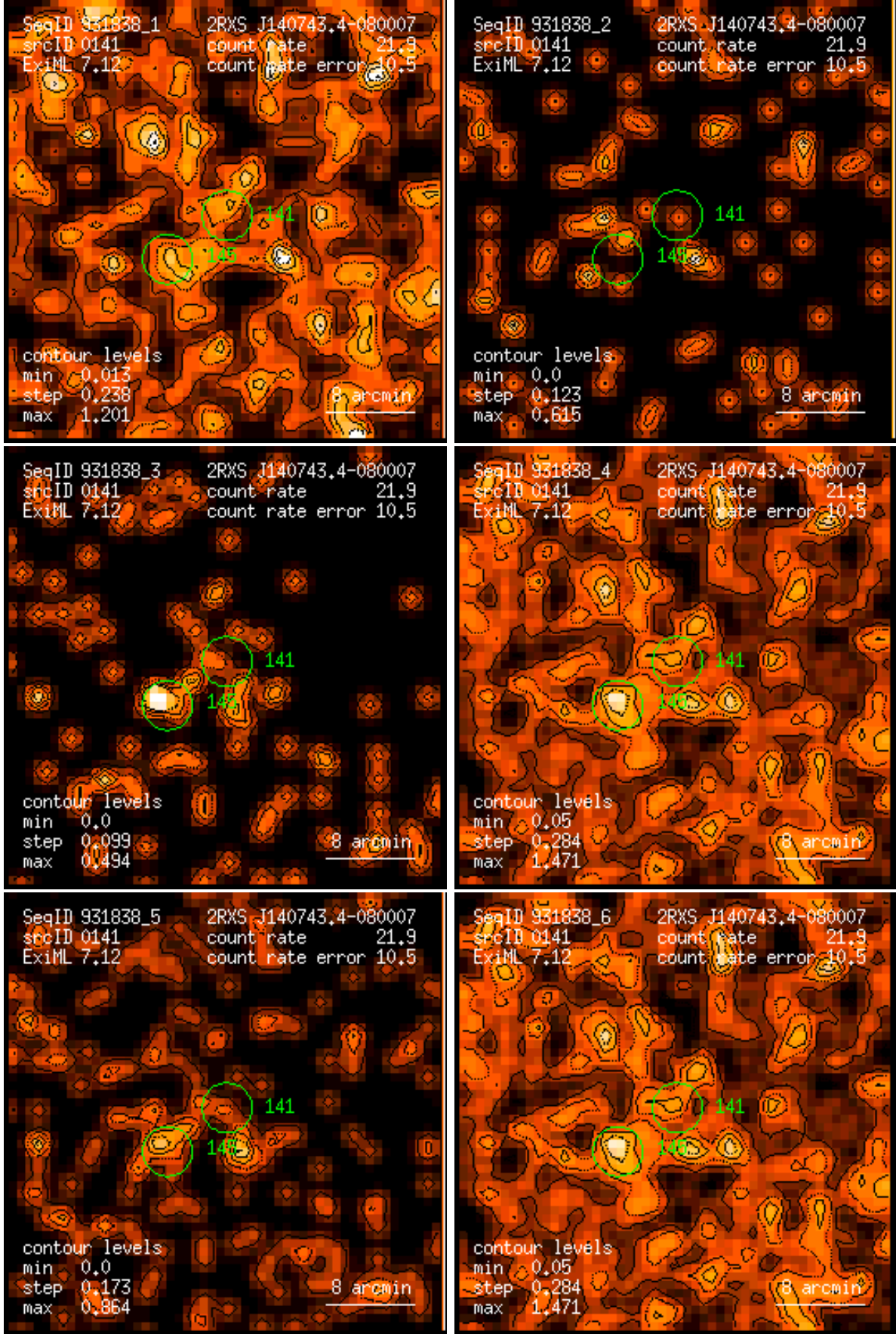
Figure 141: RASS 931838: detection 0141: band rate images, Gaussian filter: (1) PSPC channels 11 – 41, (2) 52 – 90, (3) 91 – 201, (4) 11 – 235, (5) 52 – 201, (6) 11 – 201. Broad band rates in counts/ks. Band rate contour levels in counts/ks/arcmin 2 .
