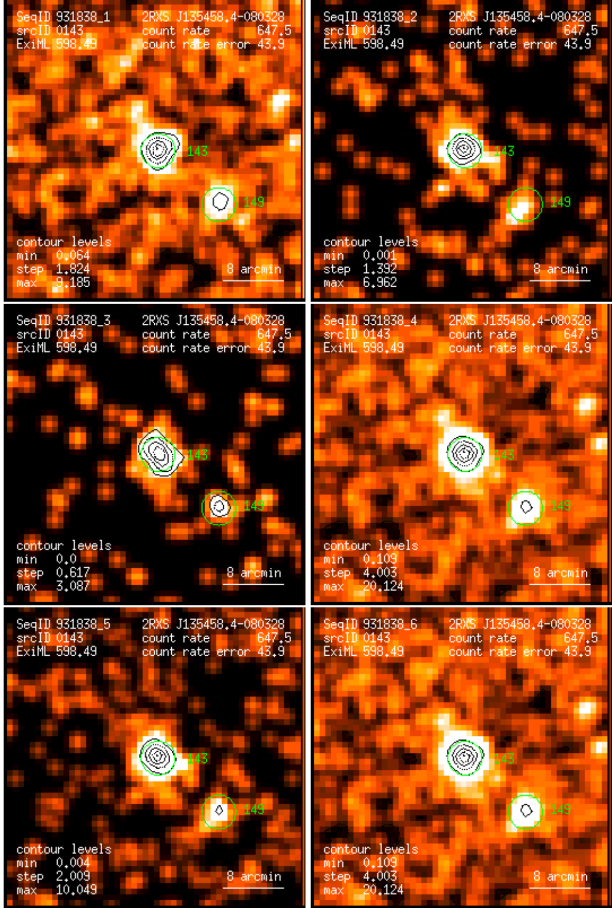
Figure 143: RASS 931838: detection 0143: band rate images, Gaussian filter: (1) PSPC channels 11 – 41, (2) 52 – 90, (3) 91 – 201, (4) 11 – 235, (5) 52 – 201, (6) 11 – 201. Broad band rates in counts/ks. Band rate contour levels in counts/ks/arcmin 2 .
