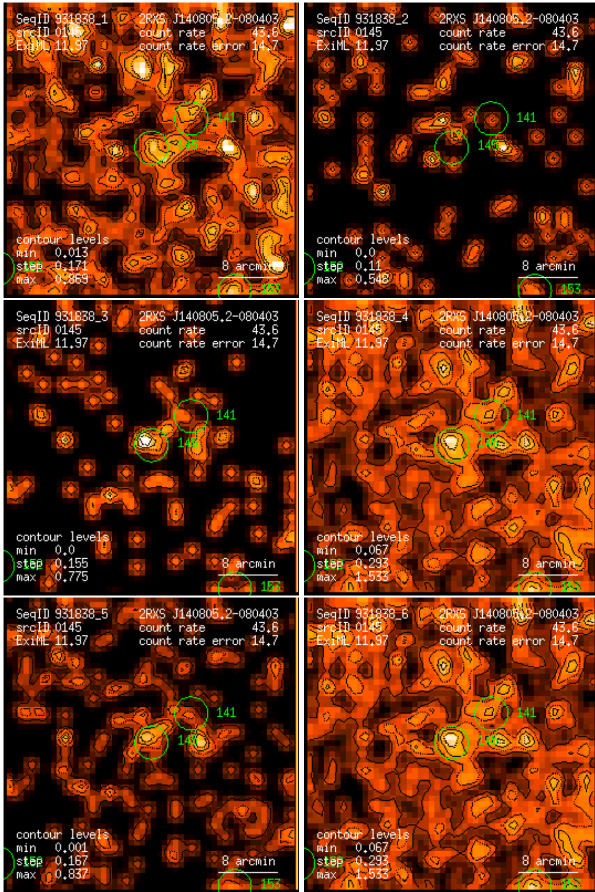
Figure 145: RASS 931838: detection 0145: band rate images, Gaussian filter: (1) PSPC channels 11 – 41, (2) 52 – 90, (3) 91 – 201, (4) 11 – 235, (5) 52 – 201, (6) 11 – 201. Broad band rates in counts/ks. Band rate contour levels in counts/ks/arcmin 2 .
