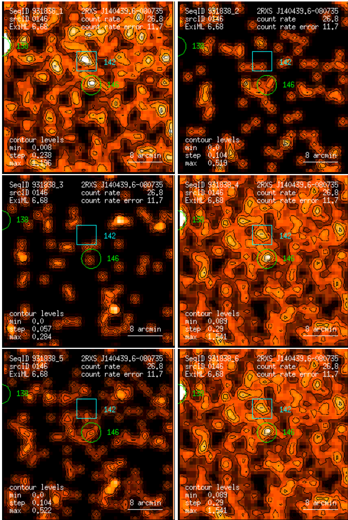
Figure 146: RASS 931838: detection 0146: band rate images, Gaussian filter: (1) PSPC channels 11 – 41, (2) 52 – 90, (3) 91 – 201, (4) 11 – 235, (5) 52 – 201, (6) 11 – 201. Broad band rates in counts/ks. Band rate contour levels in counts/ks/arcmin 2 .
