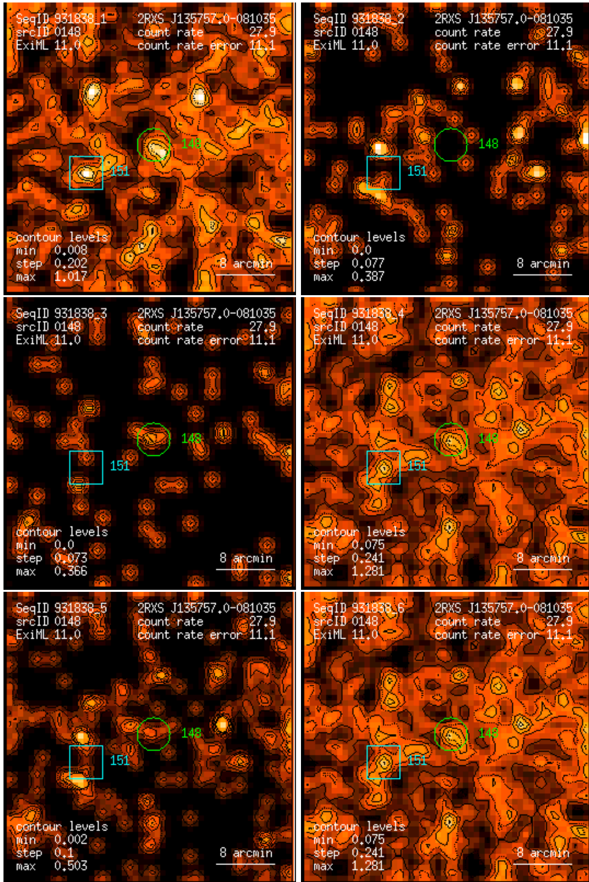
Figure 148: RASS 931838: detection 0148: band rate images, Gaussian filter: (1) PSPC channels 11 – 41, (2) 52 – 90, (3) 91 – 201, (4) 11 – 235, (5) 52 – 201, (6) 11 – 201. Broad band rates in counts/ks. Band rate contour levels in counts/ks/arcmin 2 .
