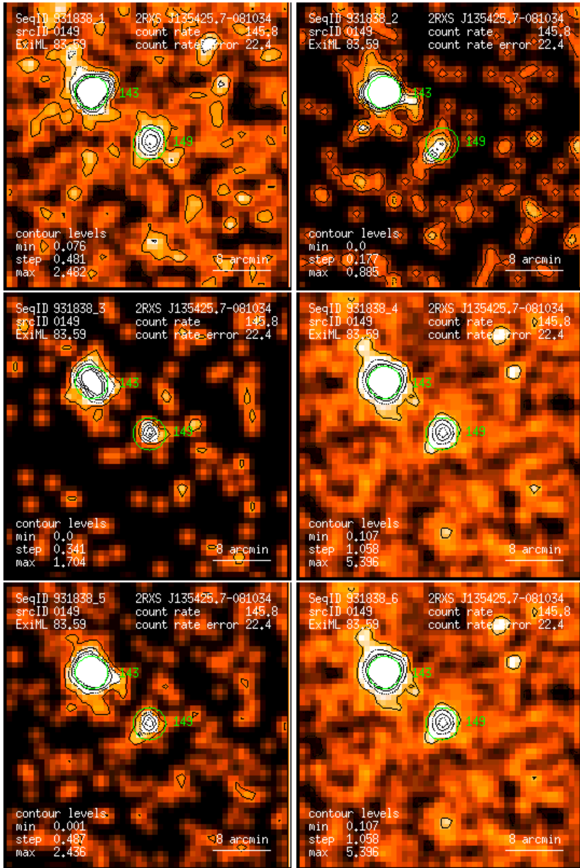
Figure 149: RASS 931838: detection 0149: band rate images, Gaussian filter: (1) PSPC channels 11 – 41, (2) 52 – 90, (3) 91 – 201, (4) 11 – 235, (5) 52 – 201, (6) 11 – 201. Broad band rates in counts/ks. Band rate contour levels in counts/ks/arcmin 2 .
