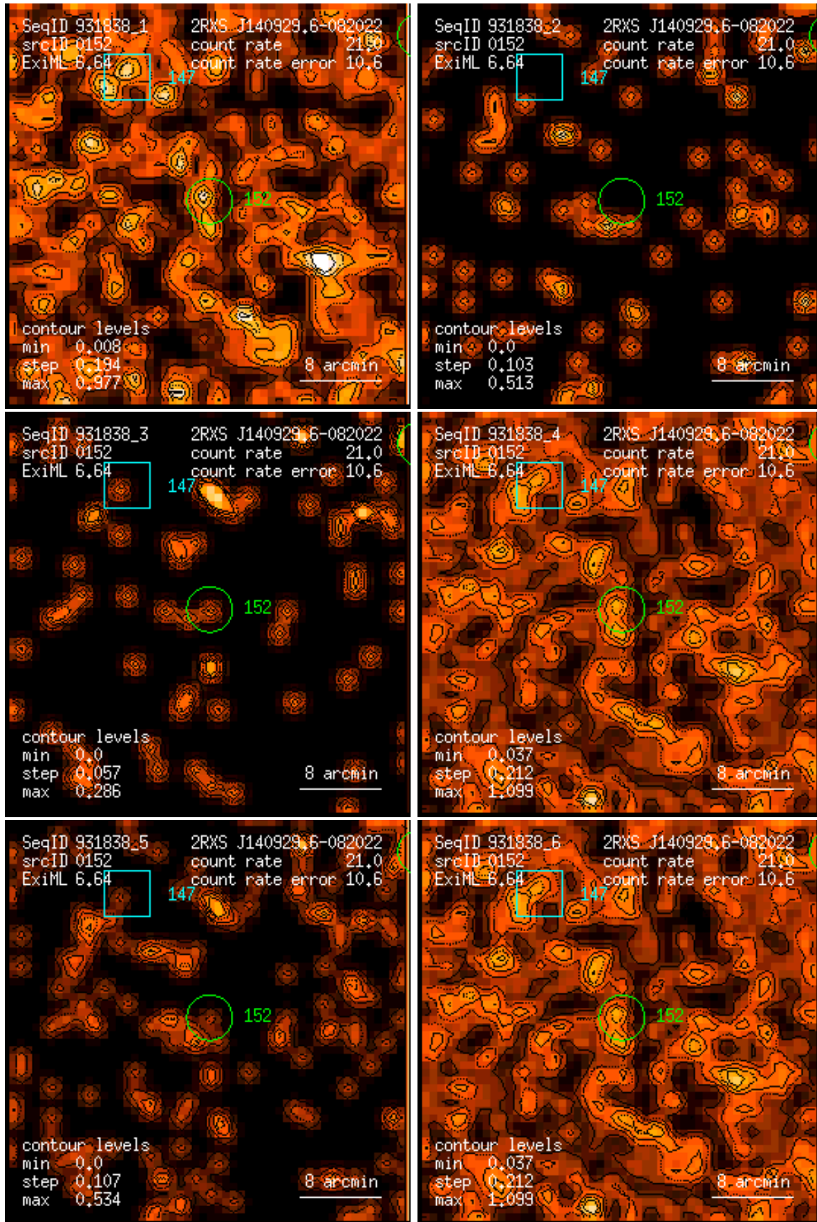
Figure 152: RASS 931838: detection 0152: band rate images, Gaussian filter: (1) PSPC channels 11 – 41, (2) 52 – 90, (3) 91 – 201, (4) 11 – 235, (5) 52 – 201, (6) 11 – 201. Broad band rates in counts/ks. Band rate contour levels in counts/ks/arcmin 2 .
