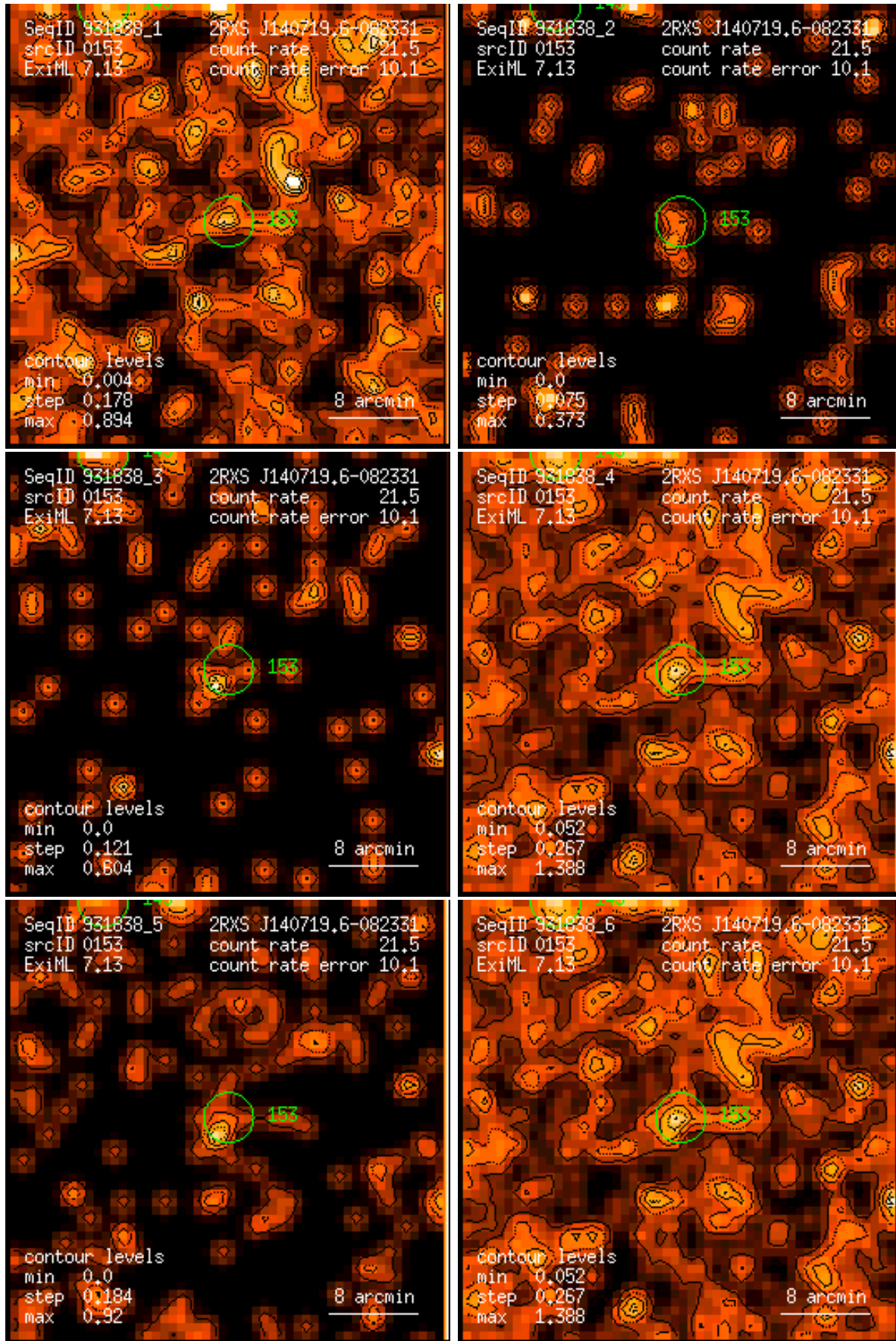
Figure 153: RASS 931838: detection 0153: band rate images, Gaussian filter: (1) PSPC channels 11 – 41, (2) 52 – 90, (3) 91 – 201, (4) 11 – 235, (5) 52 – 201, (6) 11 – 201. Broad band rates in counts/ks. Band rate contour levels in counts/ks/arcmin 2 .
