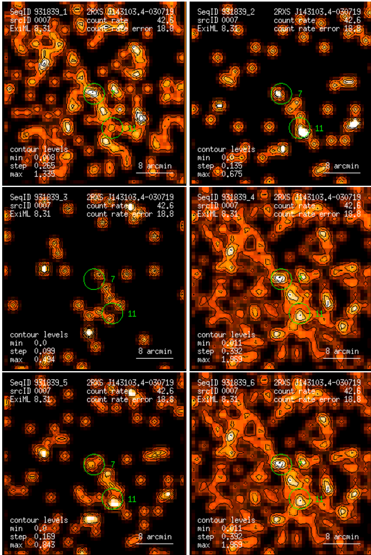
Figure 7: RASS 931839: detection 0007: band rate images, Gaussian filter: (1) PSPC channels 11 – 41, (2) 52 – 90, (3) 91 – 201, (4) 11 – 235, (5) 52 – 201, (6) 11 – 201. Broad band rates in counts/ks. Band rate contour levels in counts/ks/arcmin 2 .
