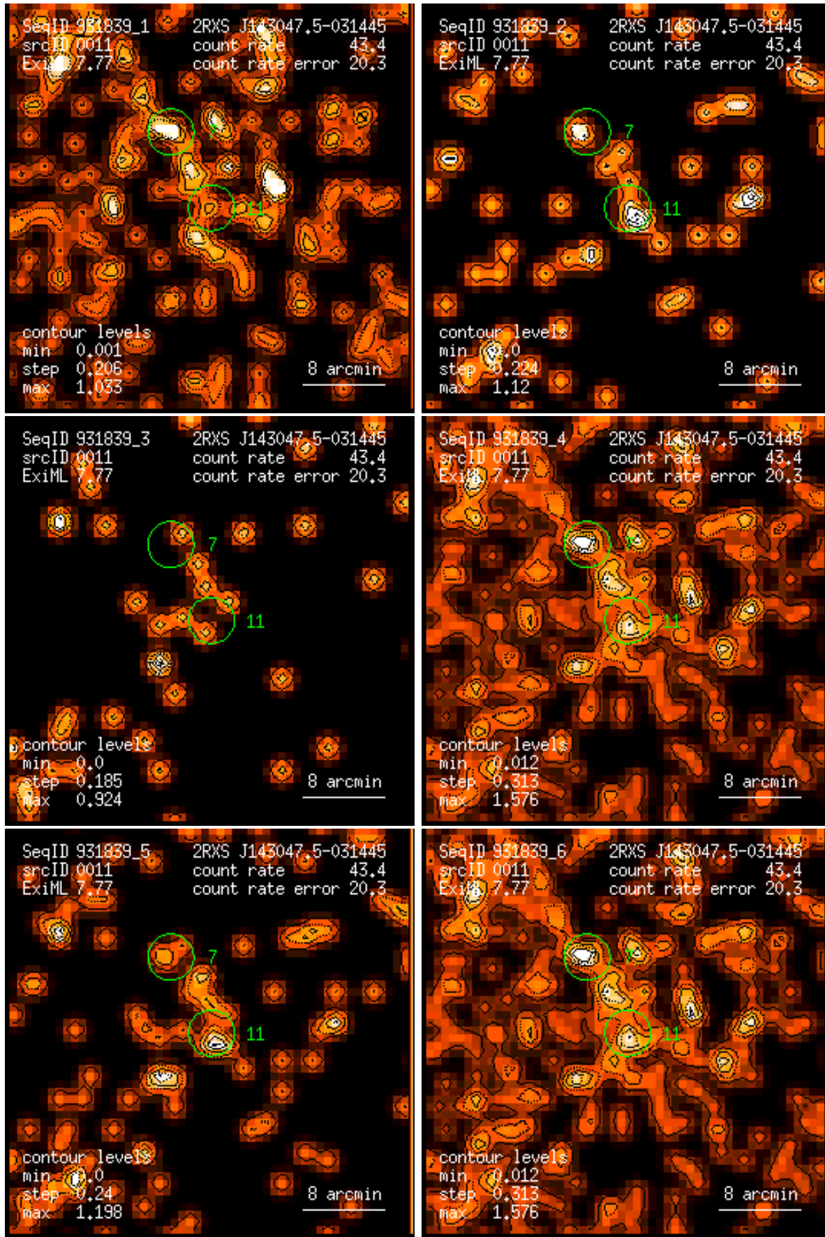
Figure 11: RASS 931839: detection 0011: band rate images, Gaussian filter: (1) PSPC channels 11 – 41, (2) 52 – 90, (3) 91 – 201, (4) 11 – 235, (5) 52 – 201, (6) 11 – 201. Broad band rates in counts/ks. Band rate contour levels in counts/ks/arcmin 2 .
