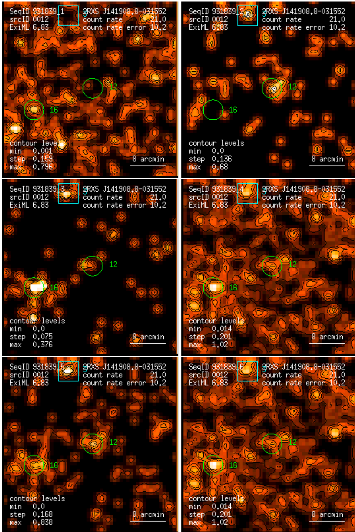
Figure 12: RASS 931839: detection 0012: band rate images, Gaussian filter: (1) PSPC channels 11 – 41, (2) 52 – 90, (3) 91 – 201, (4) 11 – 235, (5) 52 – 201, (6) 11 – 201. Broad band rates in counts/ks. Band rate contour levels in counts/ks/arcmin 2 .
