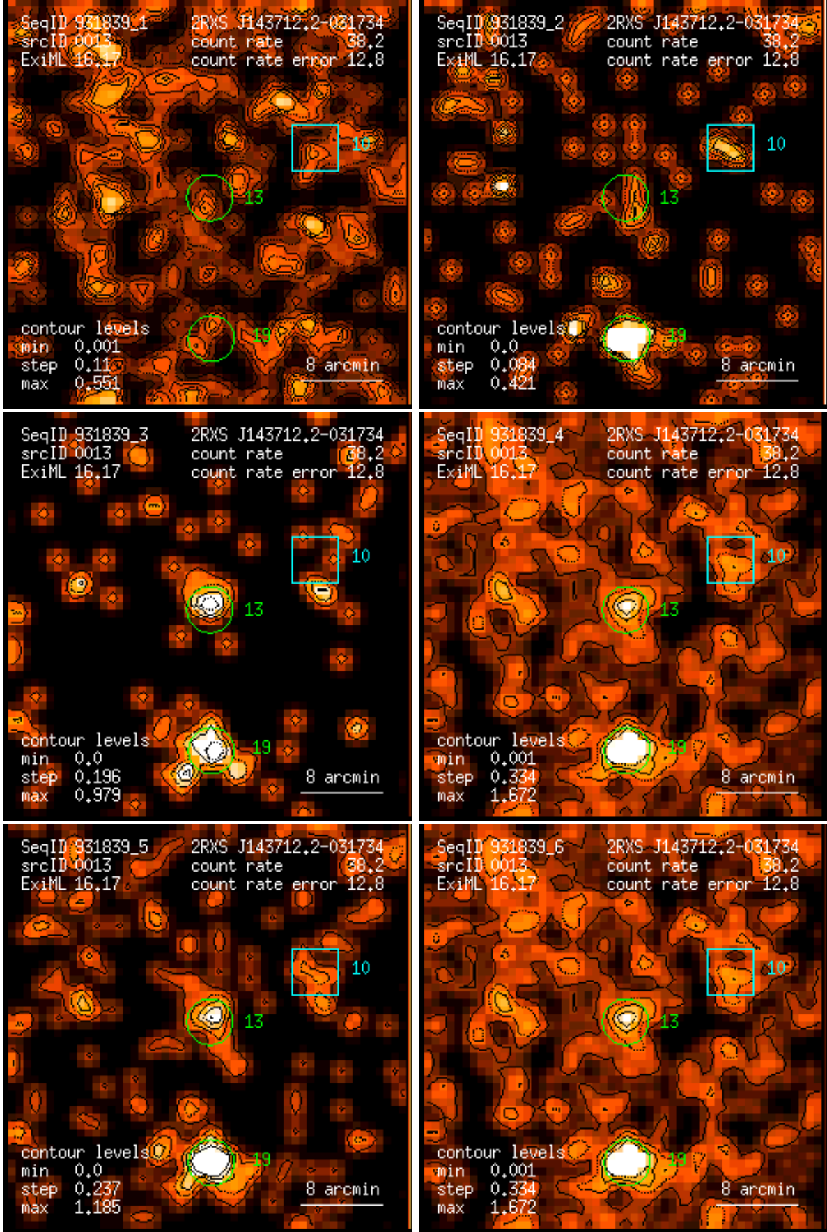
Figure 13: RASS 931839: detection 0013: band rate images, Gaussian filter: (1) PSPC channels 11 – 41, (2) 52 – 90, (3) 91 – 201, (4) 11 – 235, (5) 52 – 201, (6) 11 – 201. Broad band rates in counts/ks. Band rate contour levels in counts/ks/arcmin 2 .
