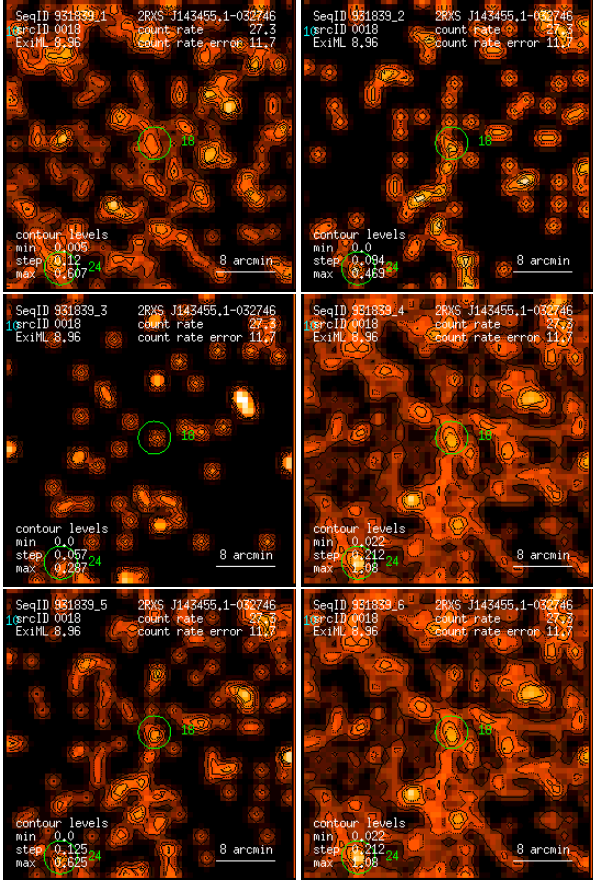
Figure 18: RASS 931839: detection 0018: band rate images, Gaussian filter: (1) PSPC channels 11 – 41, (2) 52 – 90, (3) 91 – 201, (4) 11 – 235, (5) 52 – 201, (6) 11 – 201. Broad band rates in counts/ks. Band rate contour levels in counts/ks/arcmin 2 .
