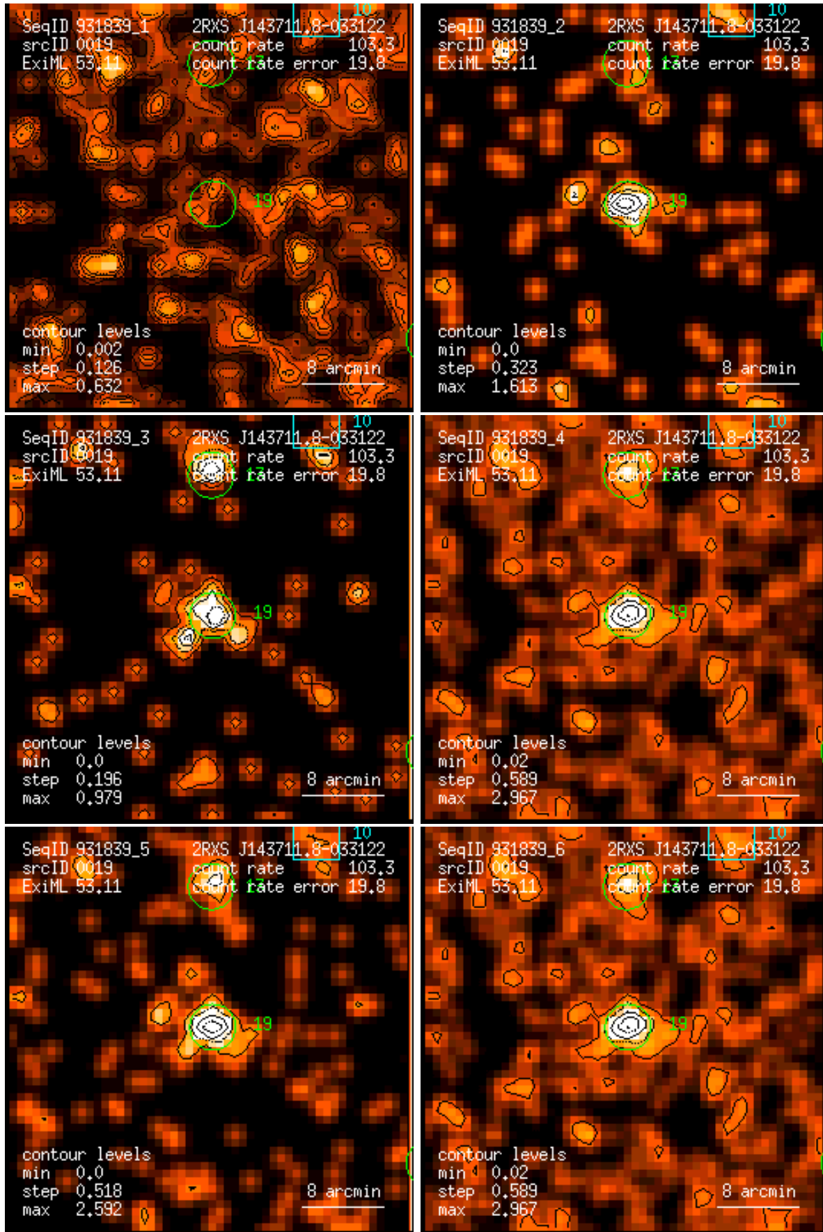
Figure 19: RASS 931839: detection 0019: band rate images, Gaussian filter: (1) PSPC channels 11 – 41, (2) 52 – 90, (3) 91 – 201, (4) 11 – 235, (5) 52 – 201, (6) 11 – 201. Broad band rates in counts/ks. Band rate contour levels in counts/ks/arcmin 2 .
