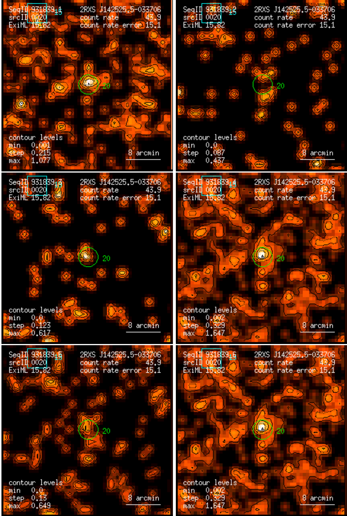
Figure 20: RASS 931839: detection 0020: band rate images, Gaussian filter: (1) PSPC channels 11 – 41, (2) 52 – 90, (3) 91 – 201, (4) 11 – 235, (5) 52 – 201, (6) 11 – 201. Broad band rates in counts/ks. Band rate contour levels in counts/ks/arcmin 2 .
