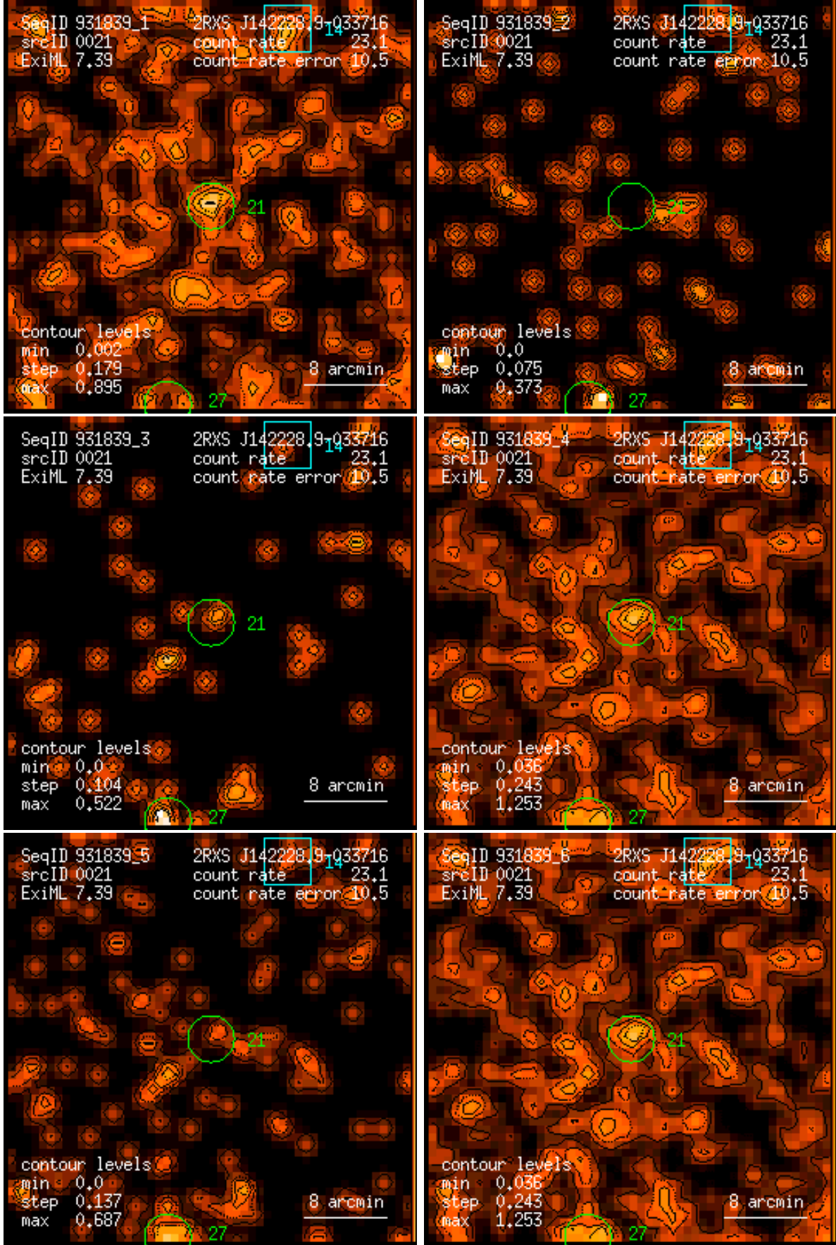
Figure 21: RASS 931839: detection 0021: band rate images, Gaussian filter: (1) PSPC channels 11 – 41, (2) 52 – 90, (3) 91 – 201, (4) 11 – 235, (5) 52 – 201, (6) 11 – 201. Broad band rates in counts/ks. Band rate contour levels in counts/ks/arcmin 2 .
