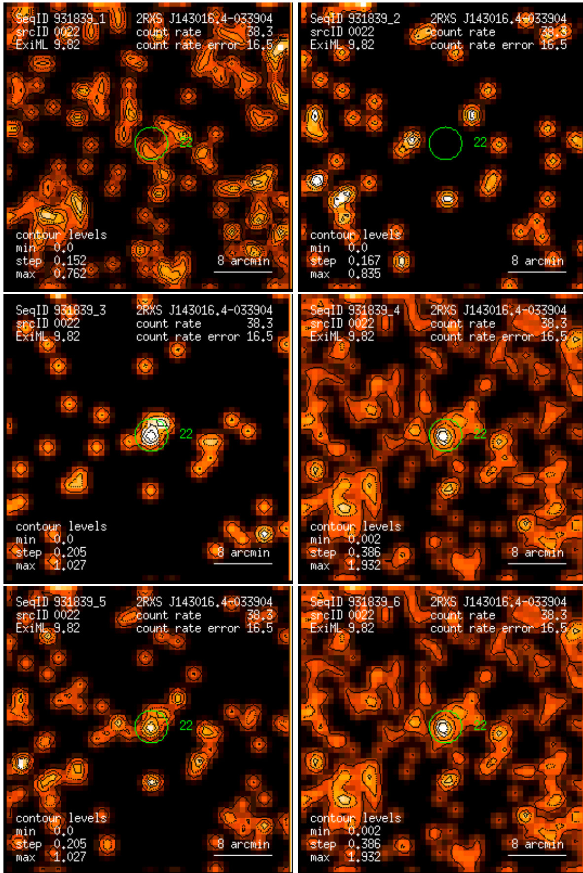
Figure 22: RASS 931839: detection 0022: band rate images, Gaussian filter: (1) PSPC channels 11 – 41, (2) 52 – 90, (3) 91 – 201, (4) 11 – 235, (5) 52 – 201, (6) 11 – 201. Broad band rates in counts/ks. Band rate contour levels in counts/ks/arcmin 2 .
