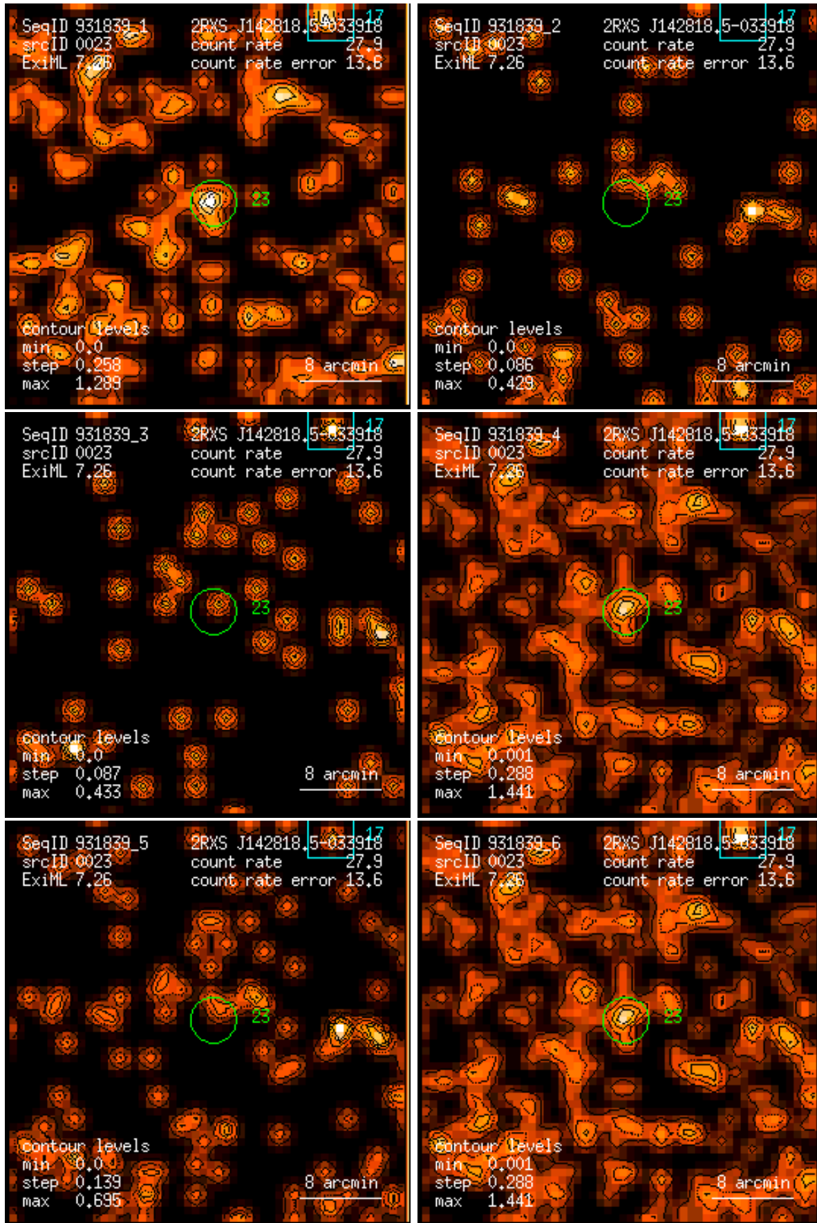
Figure 23: RASS 931839: detection 0023: band rate images, Gaussian filter: (1) PSPC channels 11 – 41, (2) 52 – 90, (3) 91 – 201, (4) 11 – 235, (5) 52 – 201, (6) 11 – 201. Broad band rates in counts/ks. Band rate contour levels in counts/ks/arcmin 2 .
