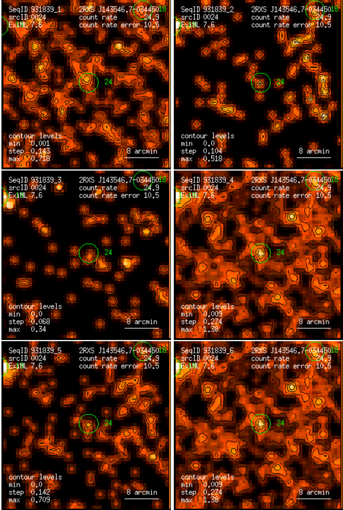
Figure 24: RASS 931839: detection 0024: band rate images, Gaussian filter: (1) PSPC channels 11 – 41, (2) 52 – 90, (3) 91 – 201, (4) 11 – 235, (5) 52 – 201, (6) 11 – 201. Broad band rates in counts/ks. Band rate contour levels in counts/ks/arcmin 2 .
