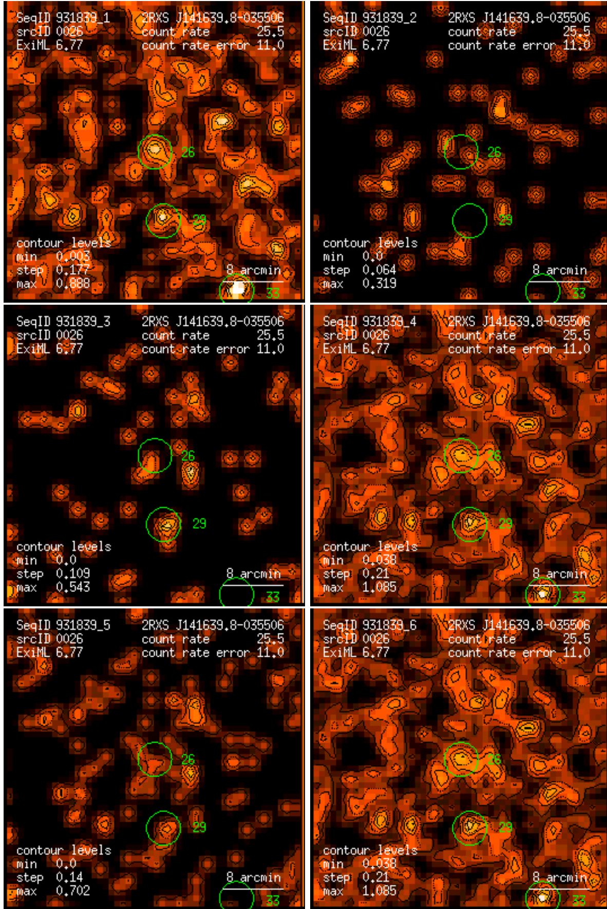
Figure 26: RASS 931839: detection 0026: band rate images, Gaussian filter: (1) PSPC channels 11 – 41, (2) 52 – 90, (3) 91 – 201, (4) 11 – 235, (5) 52 – 201, (6) 11 – 201. Broad band rates in counts/ks. Band rate contour levels in counts/ks/arcmin 2 .
