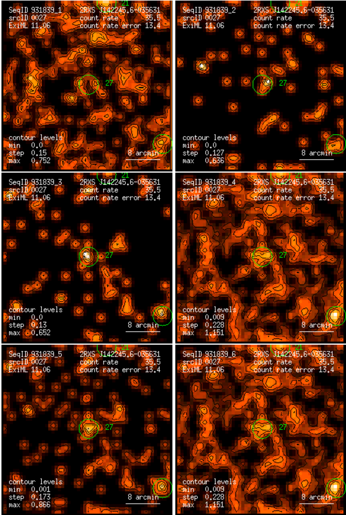
Figure 27: RASS 931839: detection 0027: band rate images, Gaussian filter: (1) PSPC channels 11 – 41, (2) 52 – 90, (3) 91 – 201, (4) 11 – 235, (5) 52 – 201, (6) 11 – 201. Broad band rates in counts/ks. Band rate contour levels in counts/ks/arcmin 2 .
