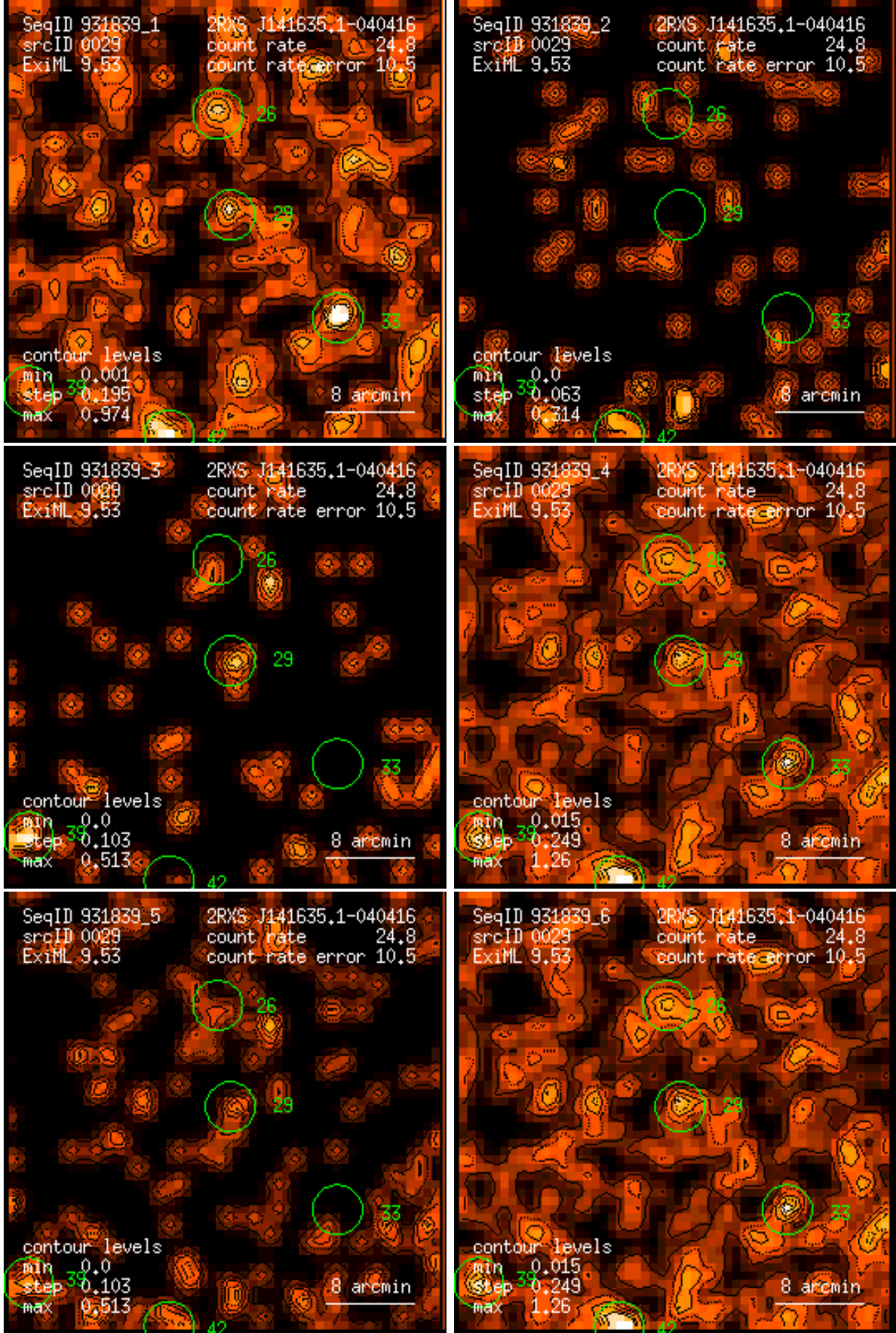
Figure 29: RASS 931839: detection 0029: band rate images, Gaussian filter: (1) PSPC channels 11 – 41, (2) 52 – 90, (3) 91 – 201, (4) 11 – 235, (5) 52 – 201, (6) 11 – 201. Broad band rates in counts/ks. Band rate contour levels in counts/ks/arcmin 2 .
