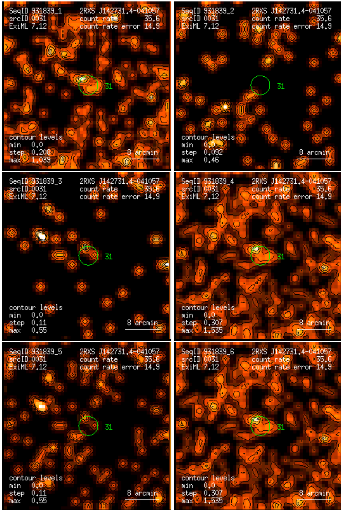
Figure 31: RASS 931839: detection 0031: band rate images, Gaussian filter: (1) PSPC channels 11 – 41, (2) 52 – 90, (3) 91 – 201, (4) 11 – 235, (5) 52 – 201, (6) 11 – 201. Broad band rates in counts/ks. Band rate contour levels in counts/ks/arcmin 2 .
