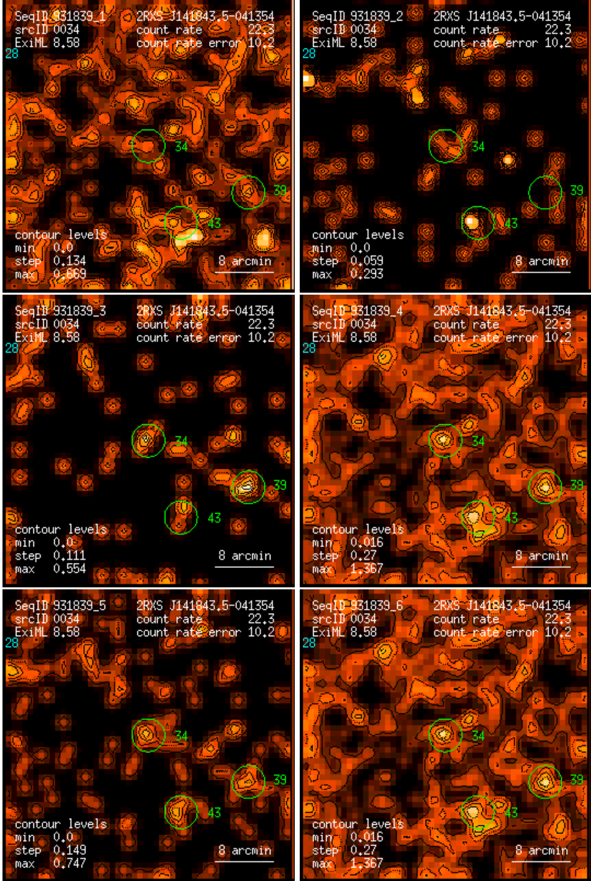
Figure 34: RASS 931839: detection 0034: band rate images, Gaussian filter: (1) PSPC channels 11 – 41, (2) 52 – 90, (3) 91 – 201, (4) 11 – 235, (5) 52 – 201, (6) 11 – 201. Broad band rates in counts/ks. Band rate contour levels in counts/ks/arcmin 2 .
