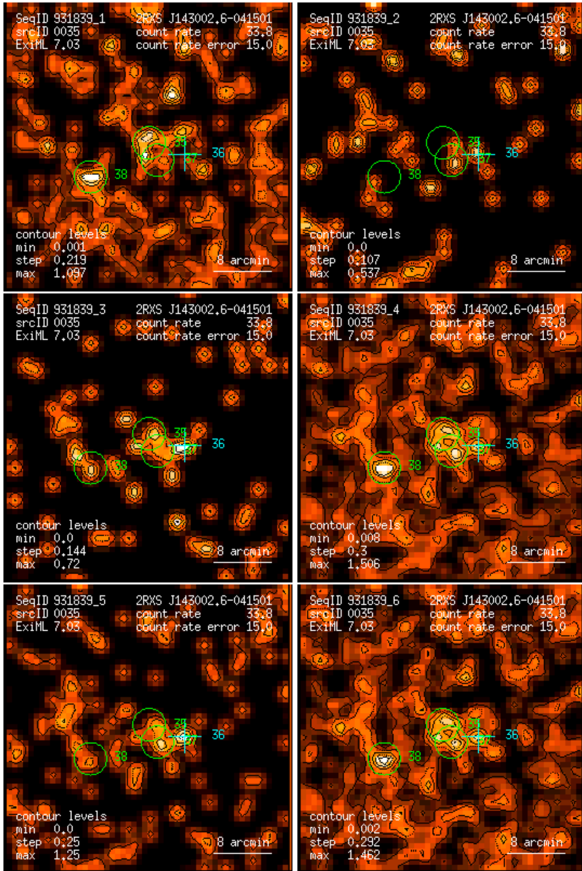
Figure 35: RASS 931839: detection 0035: band rate images, Gaussian filter: (1) PSPC channels 11 – 41, (2) 52 – 90, (3) 91 – 201, (4) 11 – 235, (5) 52 – 201, (6) 11 – 201. Broad band rates in counts/ks. Band rate contour levels in counts/ks/arcmin 2 .
