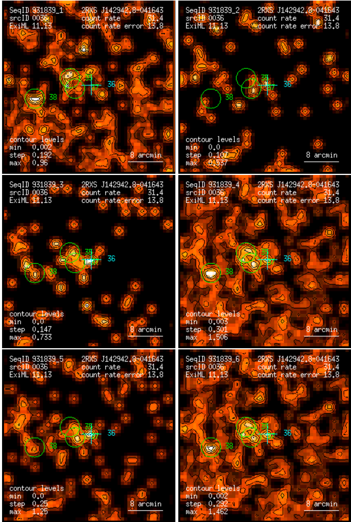
Figure 36: RASS 931839: detection 0036: band rate images, Gaussian filter: (1) PSPC channels 11 – 41, (2) 52 – 90, (3) 91 – 201, (4) 11 – 235, (5) 52 – 201, (6) 11 – 201. Broad band rates in counts/ks. Band rate contour levels in counts/ks/arcmin 2 .
