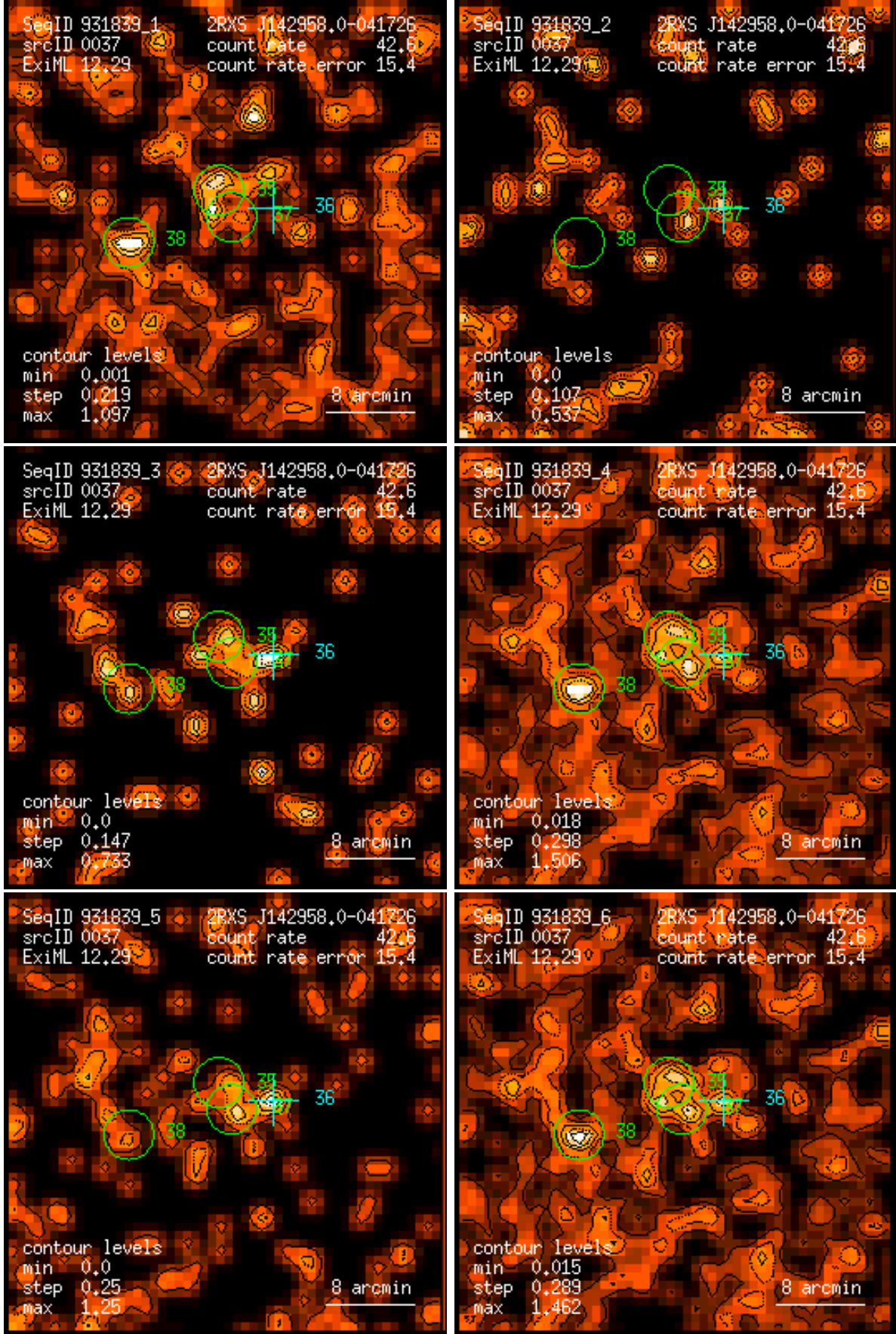
Figure 37: RASS 931839: detection 0037: band rate images, Gaussian filter: (1) PSPC channels 11 – 41, (2) 52 – 90, (3) 91 – 201, (4) 11 – 235, (5) 52 – 201, (6) 11 – 201. Broad band rates in counts/ks. Band rate contour levels in counts/ks/arcmin 2 .
