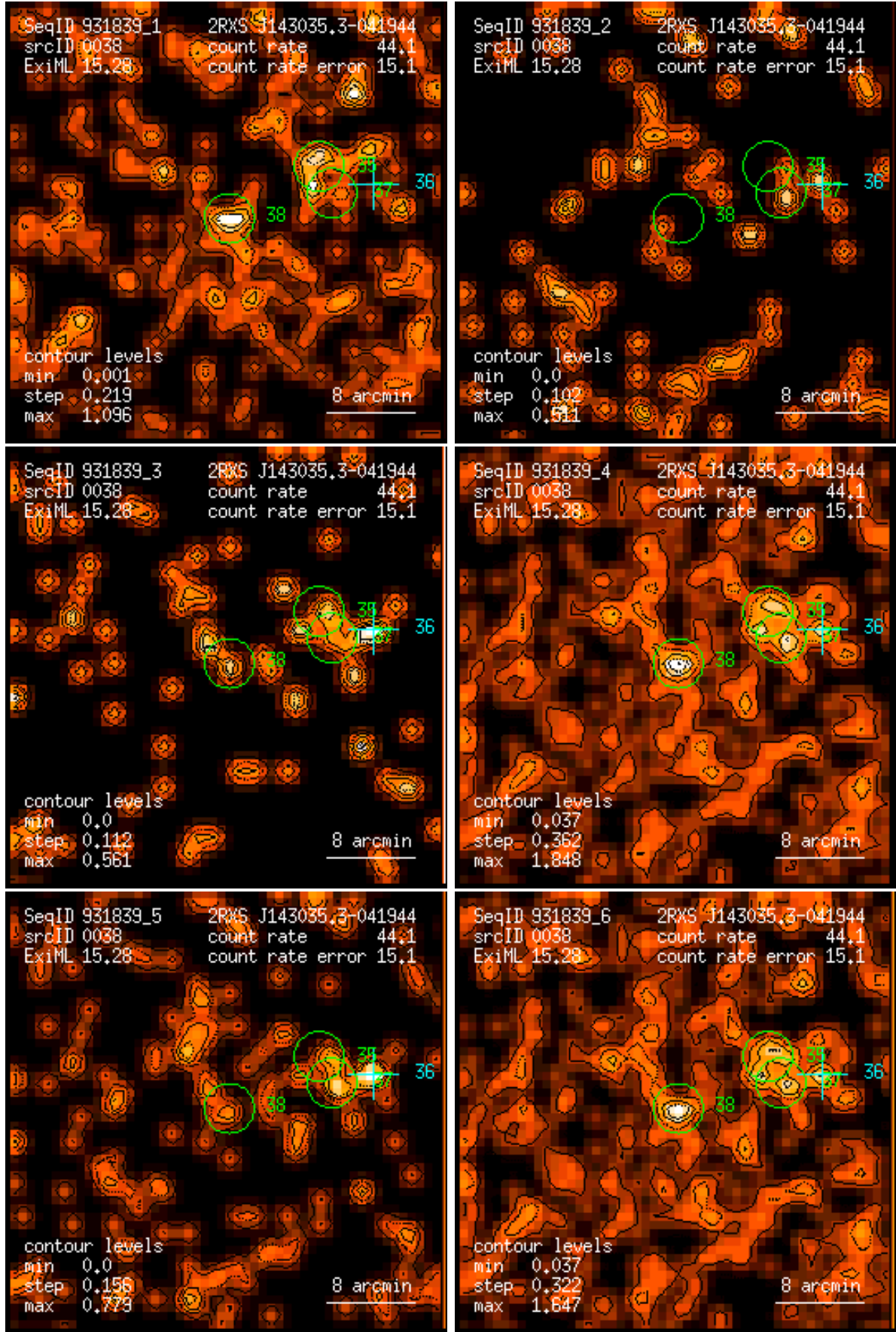
Figure 38: RASS 931839: detection 0038: band rate images, Gaussian filter: (1) PSPC channels 11 – 41, (2) 52 – 90, (3) 91 – 201, (4) 11 – 235, (5) 52 – 201, (6) 11 – 201. Broad band rates in counts/ks. Band rate contour levels in counts/ks/arcmin 2 .
