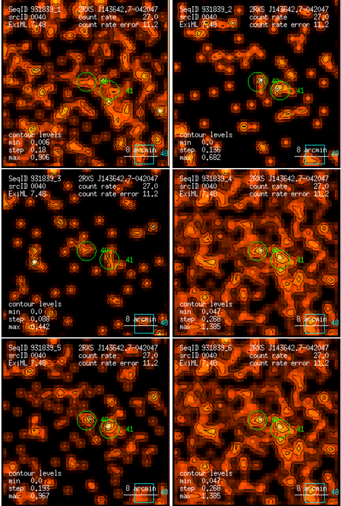
Figure 40: RASS 931839: detection 0040: band rate images, Gaussian filter: (1) PSPC channels 11 – 41, (2) 52 – 90, (3) 91 – 201, (4) 11 – 235, (5) 52 – 201, (6) 11 – 201. Broad band rates in counts/ks. Band rate contour levels in counts/ks/arcmin 2 .
