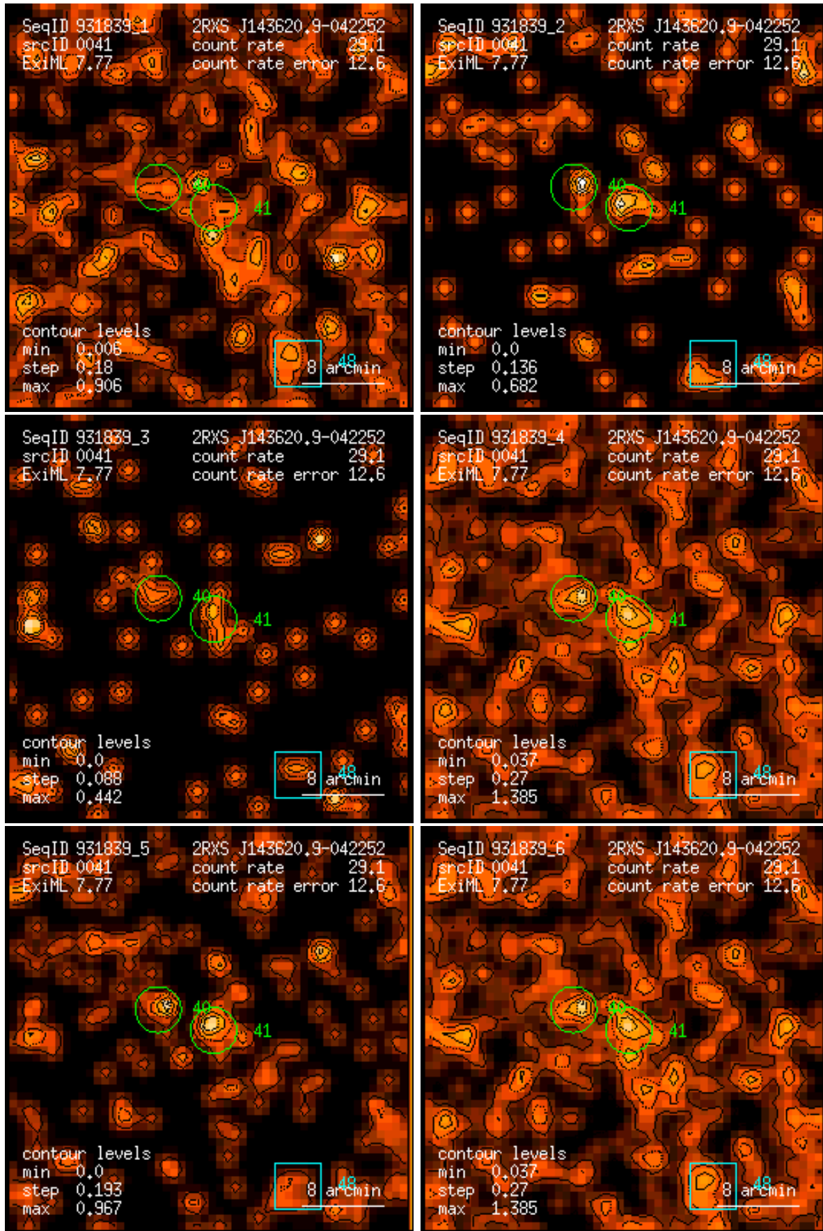
Figure 41: RASS 931839: detection 0041: band rate images, Gaussian filter: (1) PSPC channels 11 – 41, (2) 52 – 90, (3) 91 – 201, (4) 11 – 235, (5) 52 – 201, (6) 11 – 201. Broad band rates in counts/ks. Band rate contour levels in counts/ks/arcmin 2 .
