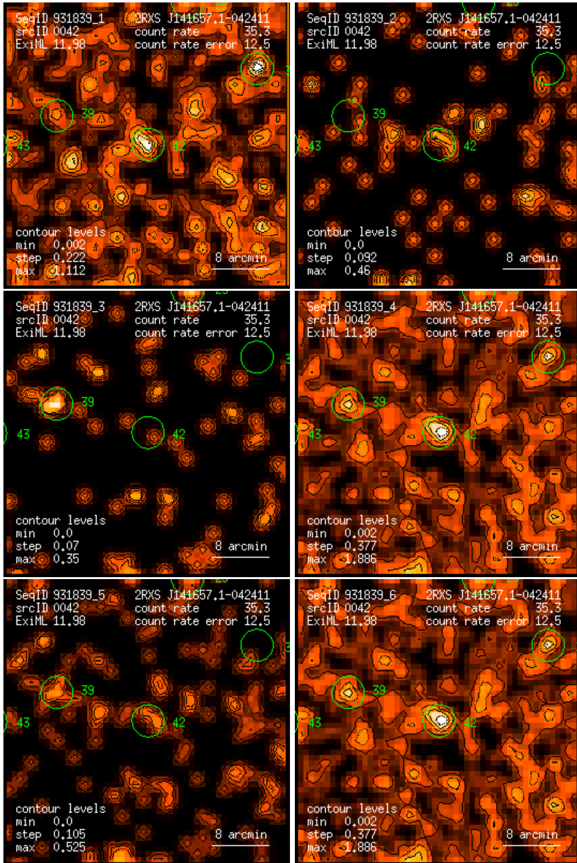
Figure 42: RASS 931839: detection 0042: band rate images, Gaussian filter: (1) PSPC channels 11 – 41, (2) 52 – 90, (3) 91 – 201, (4) 11 – 235, (5) 52 – 201, (6) 11 – 201. Broad band rates in counts/ks. Band rate contour levels in counts/ks/arcmin 2 .
