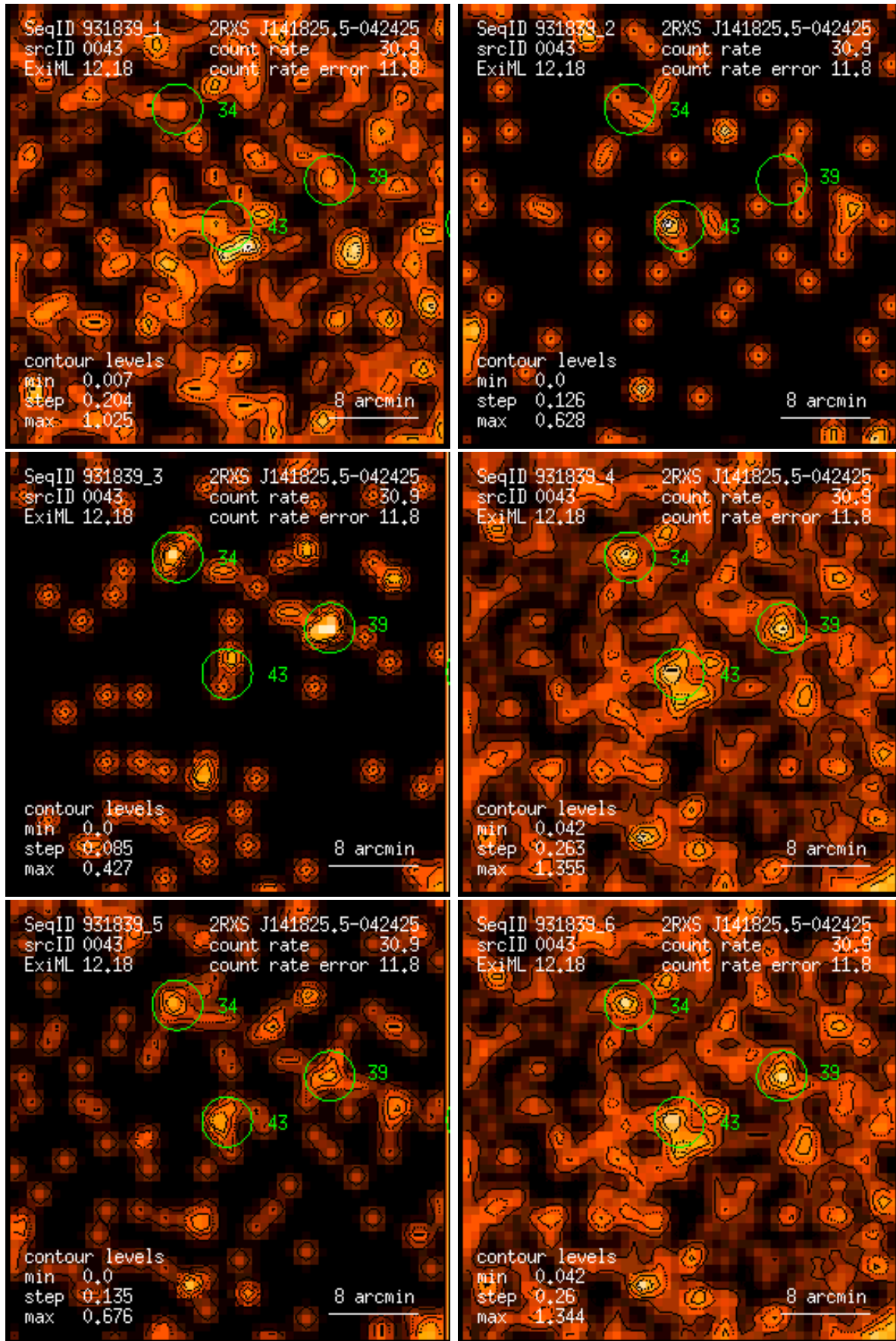
Figure 43: RASS 931839: detection 0043: band rate images, Gaussian filter: (1) PSPC channels 11 – 41, (2) 52 – 90, (3) 91 – 201, (4) 11 – 235, (5) 52 – 201, (6) 11 – 201. Broad band rates in counts/ks. Band rate contour levels in counts/ks/arcmin 2 .
